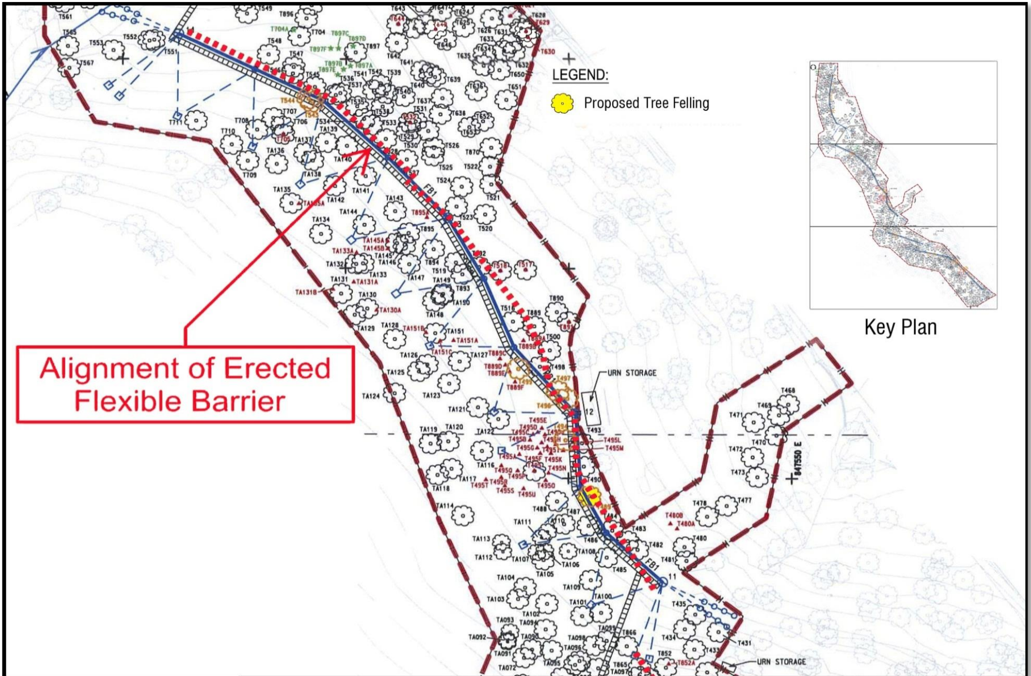
Figure 2 IEC Audit Route along the Erected Flexible Barrier on 29 July 2015 (Sheet 2 of 3)
