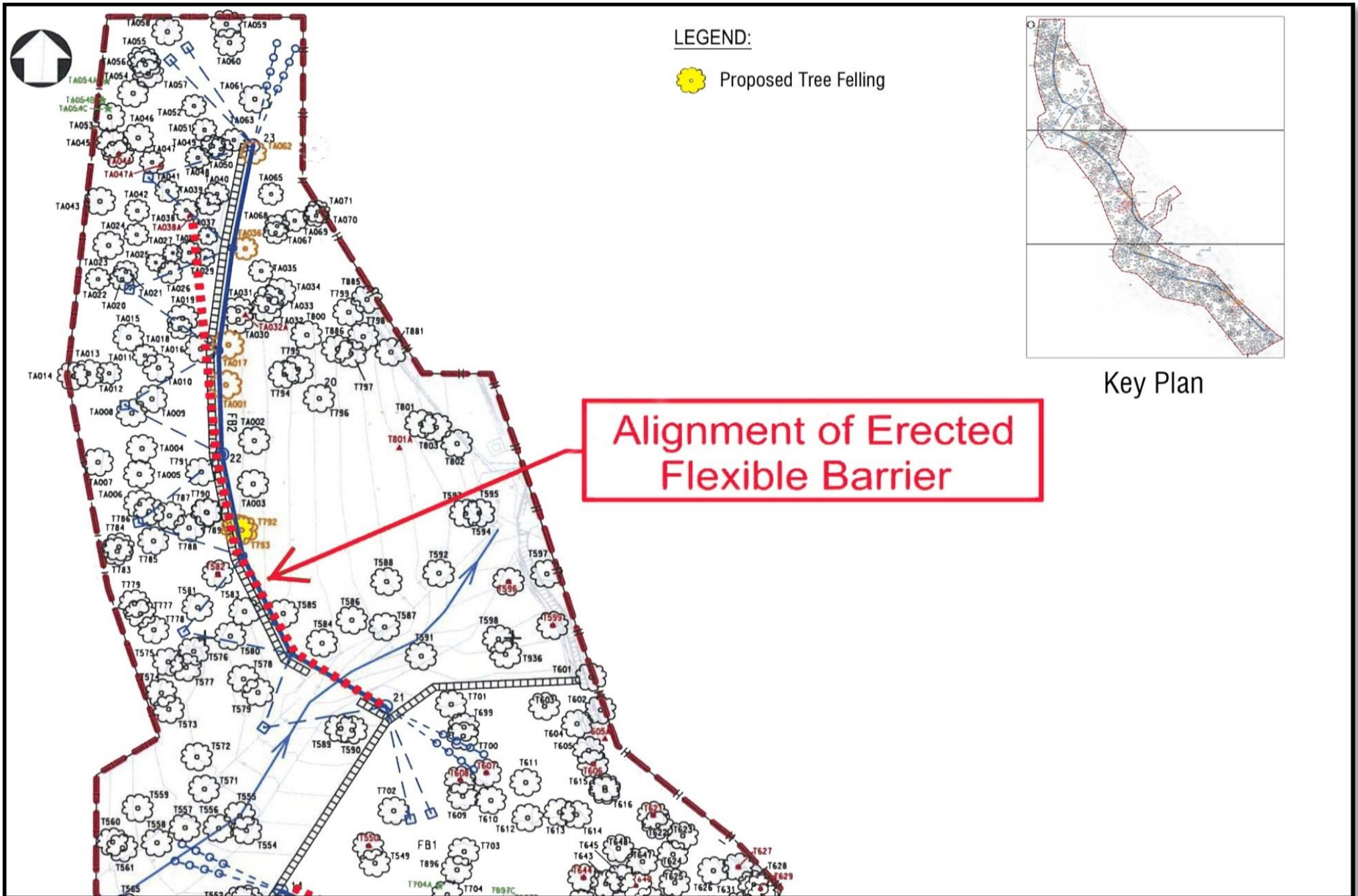
Figure 2 IEC Audit Route along the Erected Flexible Barrier on 12 January 2016 (Sheet 1 of 3)
