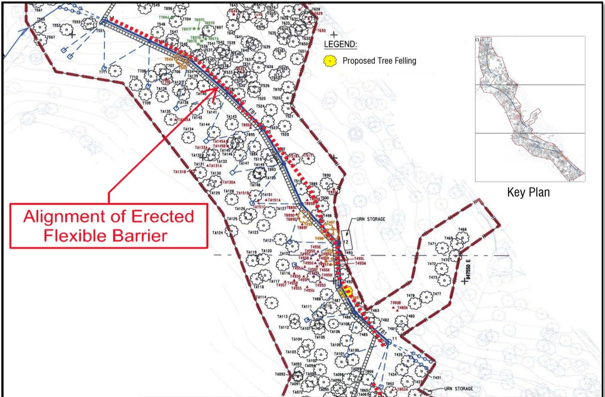
Figure 2 IEC Audit Route along the Erected Flexible Barrier on 12 January 2016 (Sheet 2 of 3)
