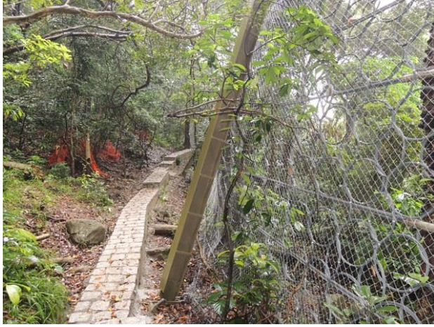
Photo 3 Completed flexible barrier
