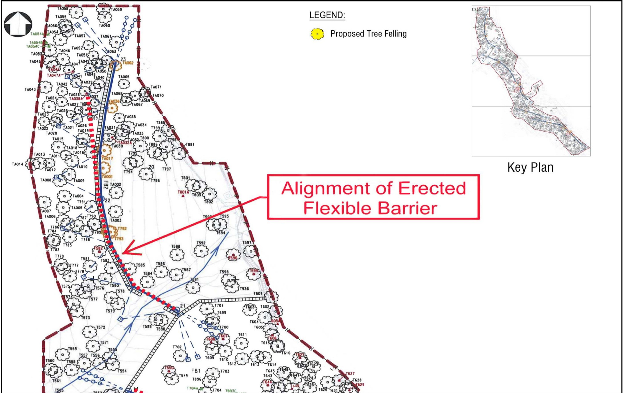
Figure 2 IEC Audit Route along the Erected Flexible Barrier on 27 April 2016 (Sheet 1 of 3)
