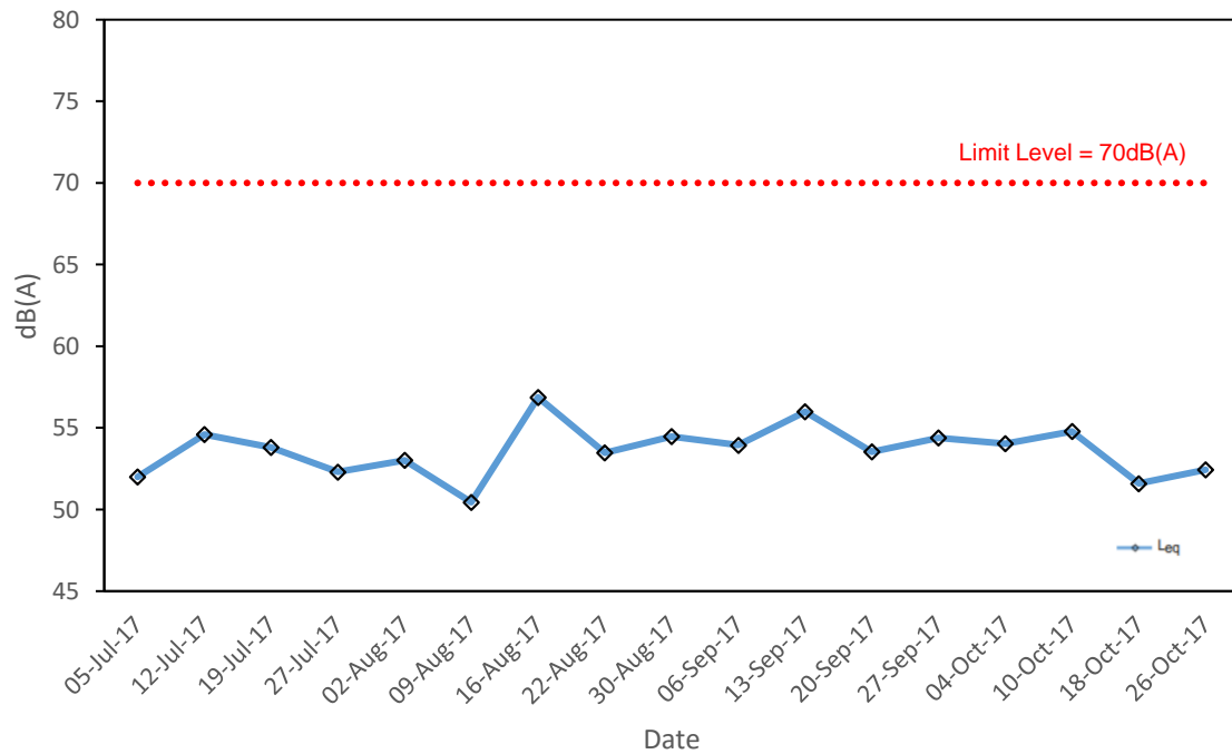
Noise Level for 30 min, dB(A), at NM2
