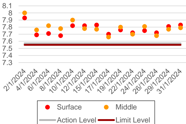
Dissolved Oxygen (Surface & Middle) during Mid-Flood
