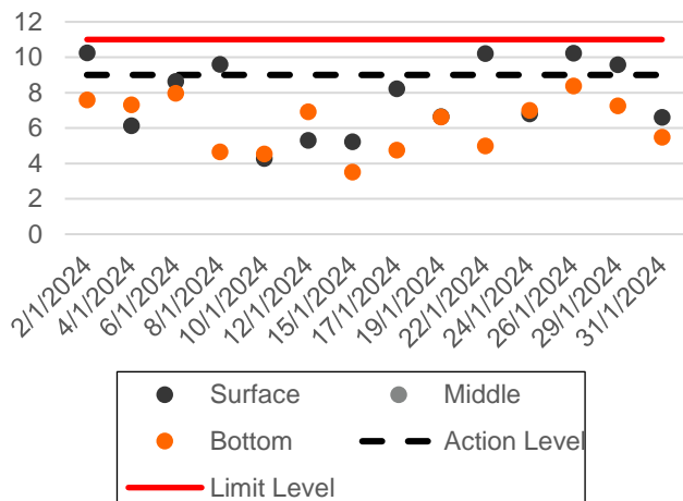
Suspended Solids (Depth Average) during Mid-Flood
