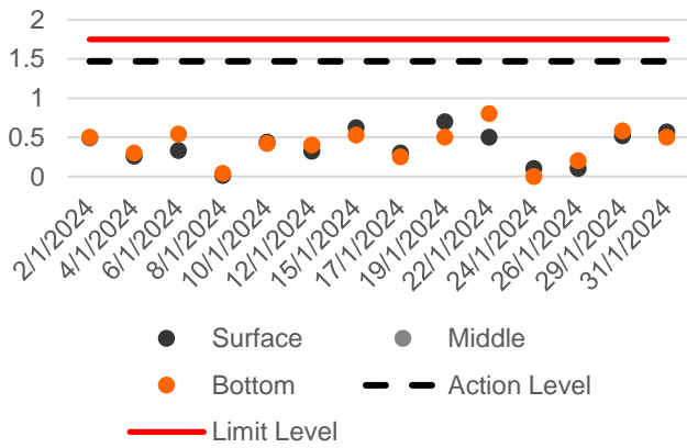
Turbidity (Depth-Averaged) during Mid-Ebb
