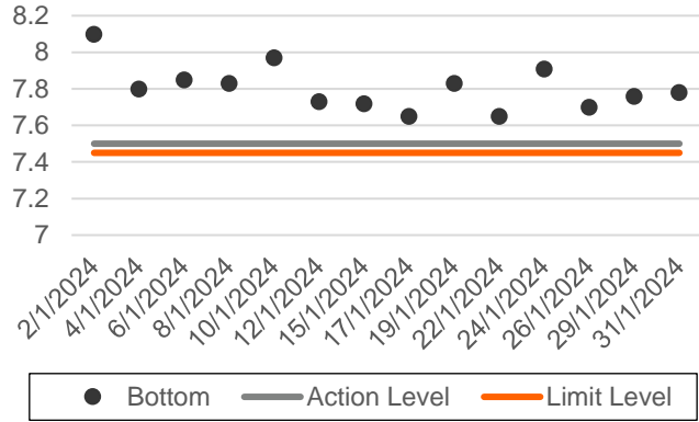
Dissolved Oxygen (Bottom) during Mid-Ebb
