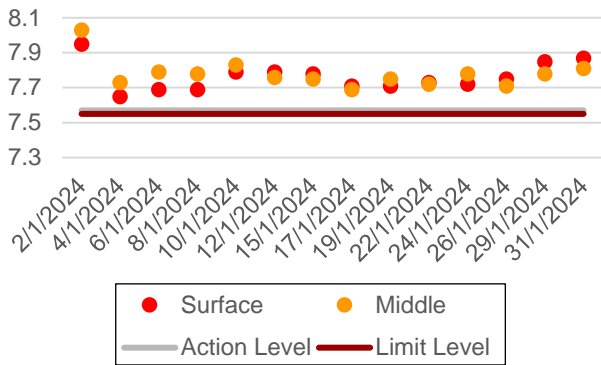
Dissolved Oxygen (Surface & Middle) during Mid-Ebb
