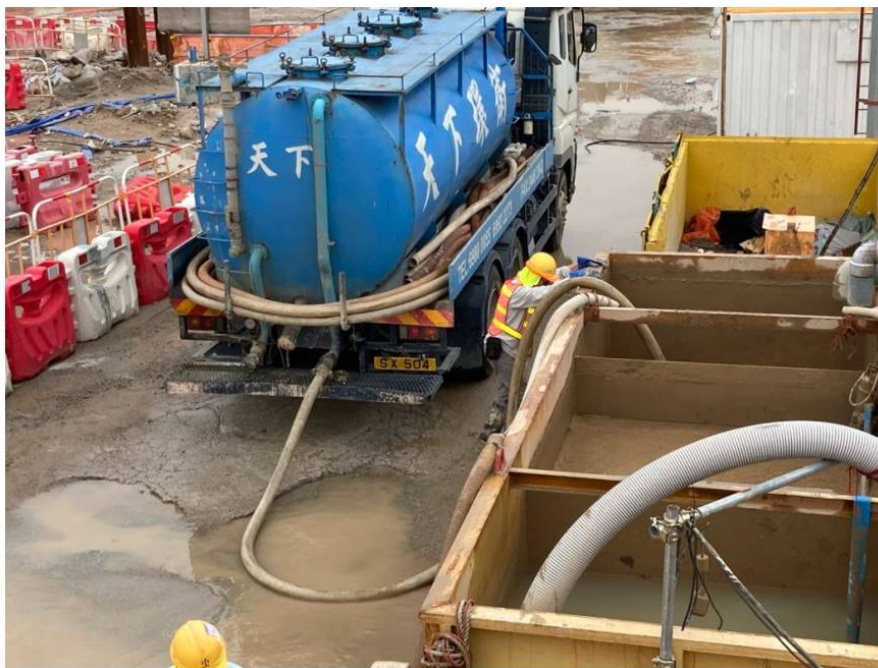
Photo 7a: Regular Sludge Removal at Sedimentation Tank
