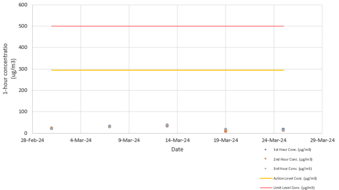
1-hour TSP concentration vs date for Location DM1
