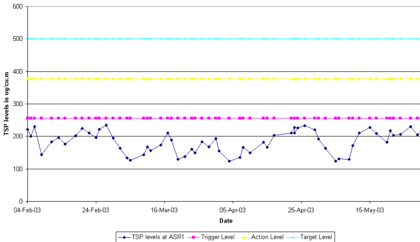
Figure 6.2 - Graphical Plot of 1-hour TSP Levels
