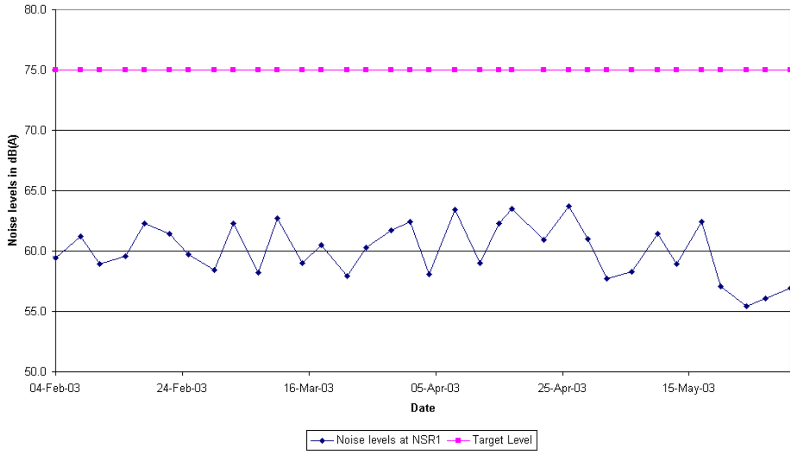
Figure 6.3 - Graphical Plot of Noise Levels
