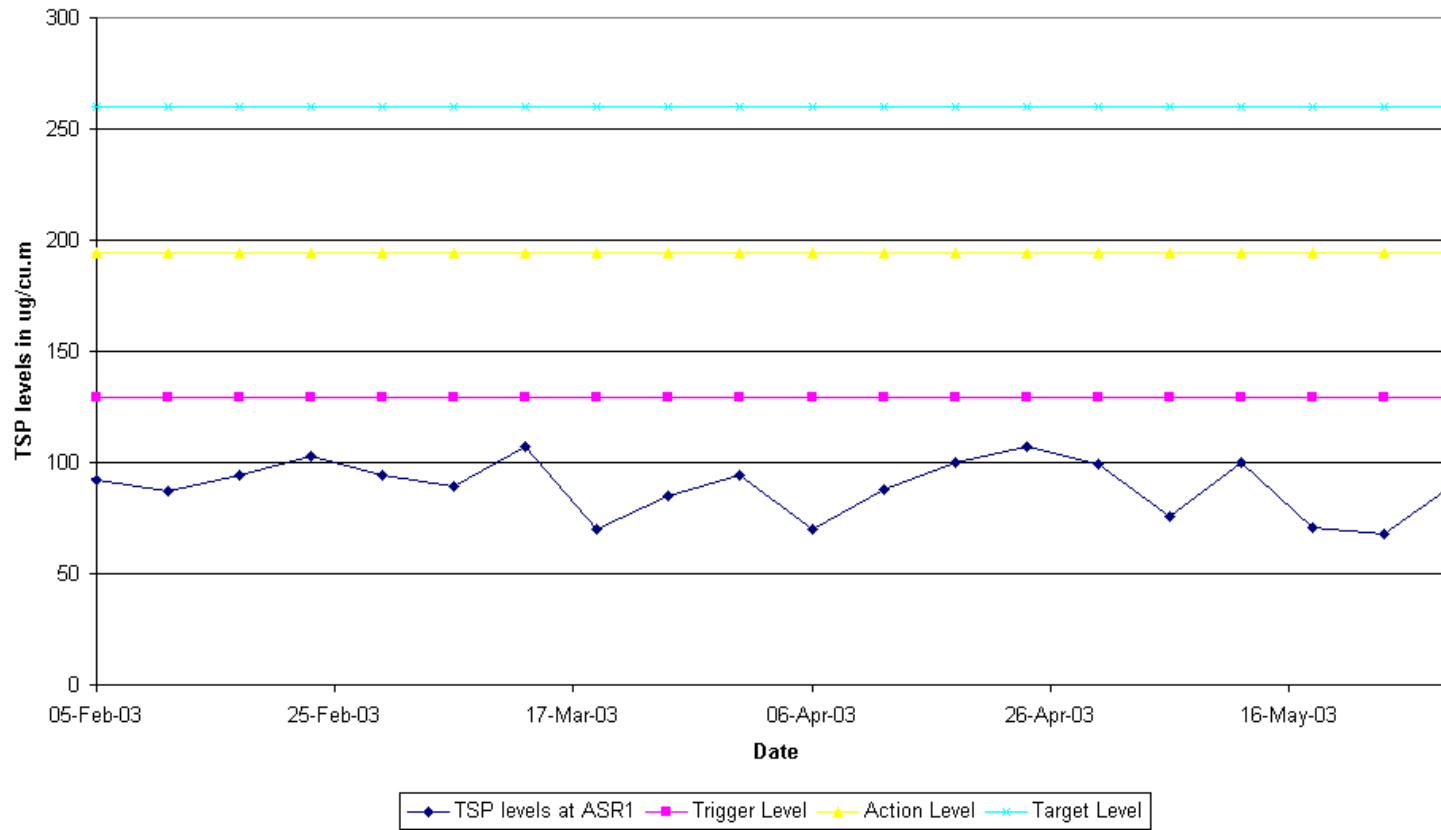
Figure 6.1 - Graphical Plot of 24-hour TSP Levels
