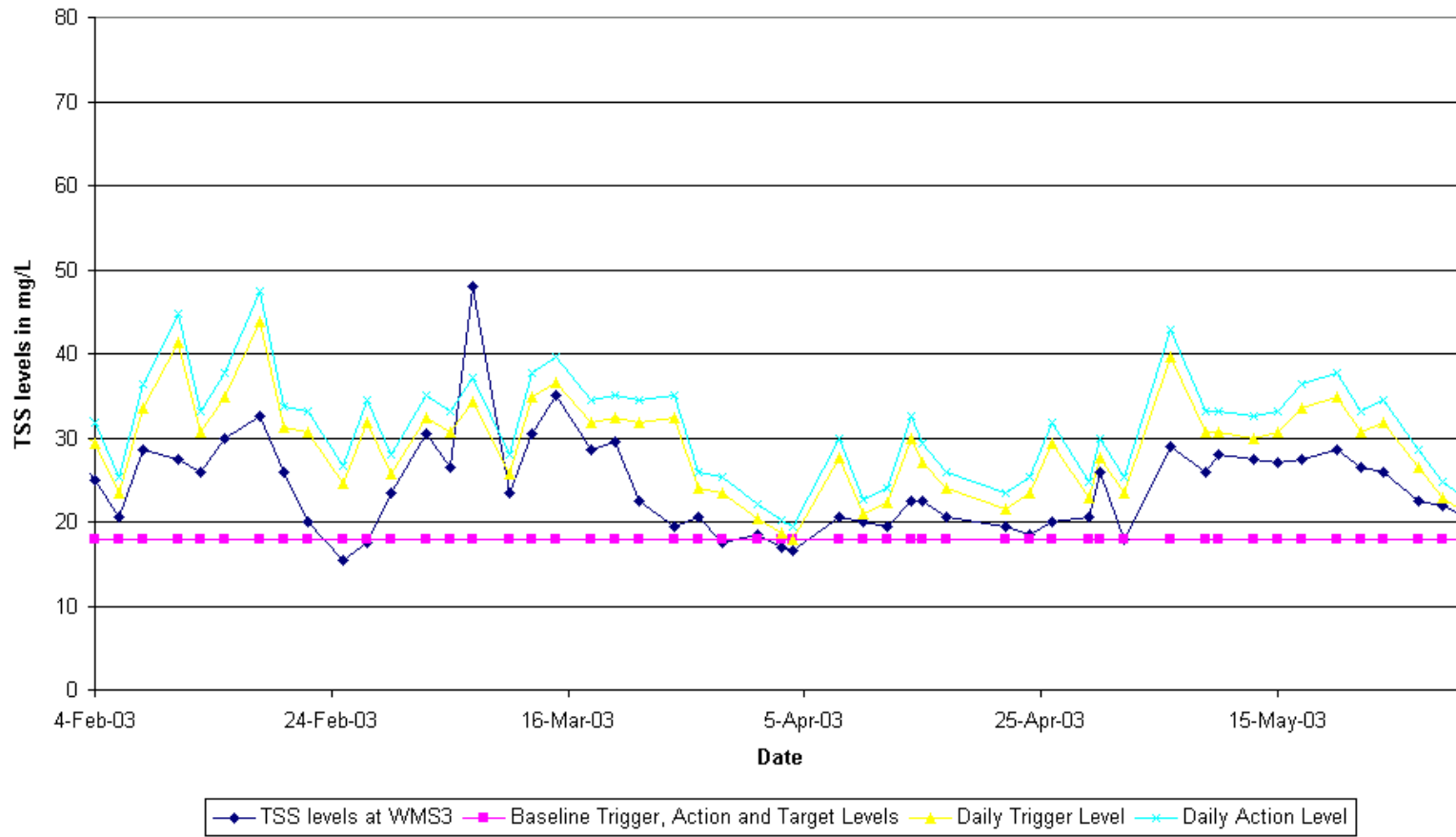
Figure 6.4 - Graphical Plot of Suspended Solids Levels
