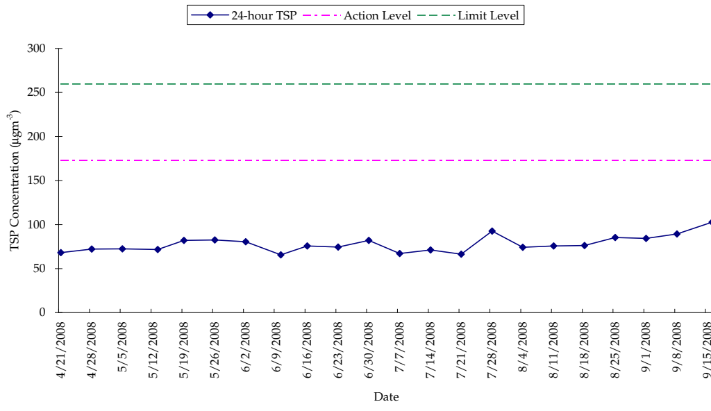
Figure F1 - Measured 24-hour TSP Concentration ( \mu\text{g}\text{m}^{-3} ) at AM1
