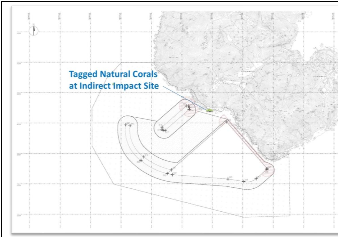
Figure 5.1 Tagged Natural Corals at Indirect Impact Site Near SKC
