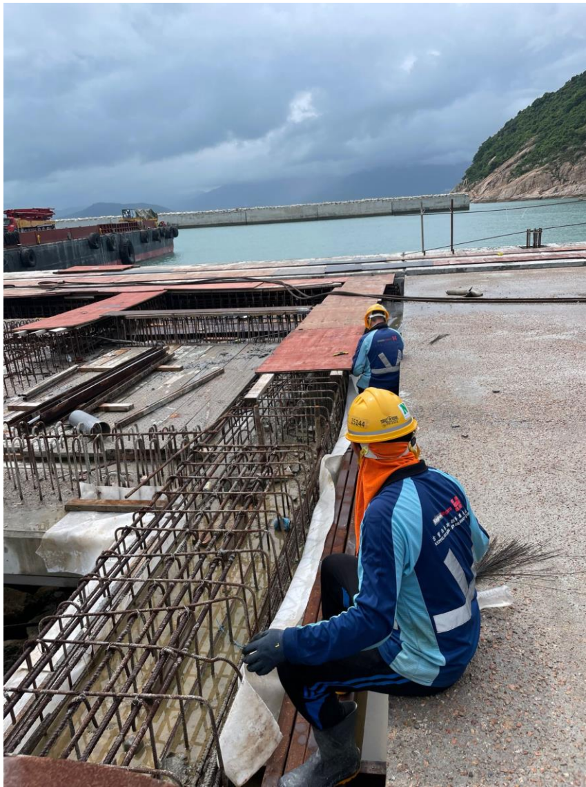
Figure 1 Replacement of Damaged Geotextile on 05 September 2023
