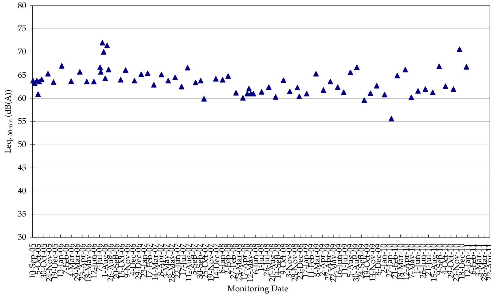
Rooftop of the Central Maintenance Building (NM4)
