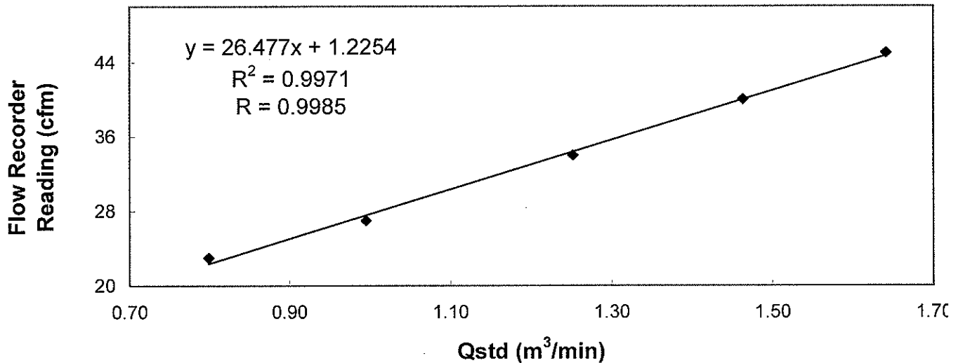
Sampler 9795 Calibration Curve Site: Wan Chai (AM-2)
