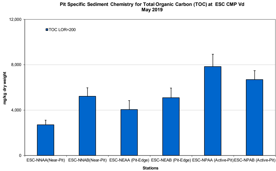
Figure 13: Concentration of Total Organic Carbon (TOC) (mg/kg dry weight; mean +SD) in sediment samples collected from Pit Specific Sediment Chemistry Monitoring for ESC CMP Vd in May 2019.
