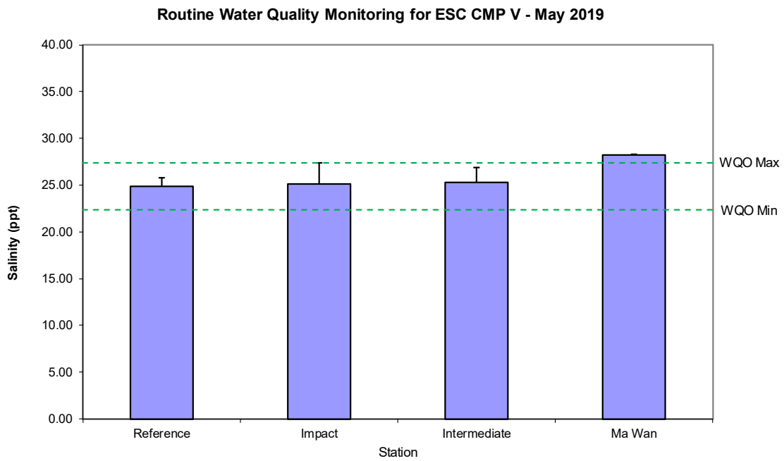
Figure 5: Level of Salinity (ppt; mean + SD) recorded during Routine Water Quality Monitoring for disposal operations at ESC CMP V in May 2019.
