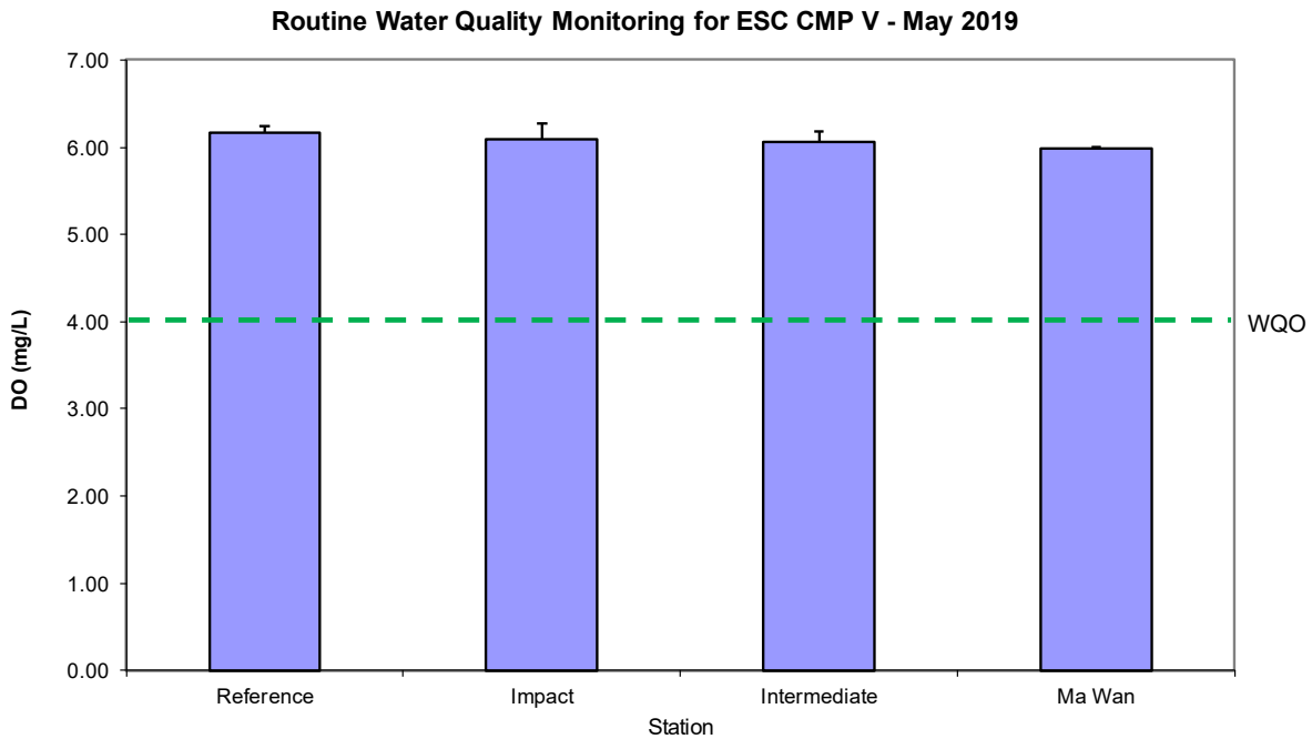
Figure 3: Concentration of Dissolved Oxygen (DO) (mg/L; mean + SD) recorded during Routine Water Quality Monitoring for disposal operations at ESC CMP V in May 2019.
