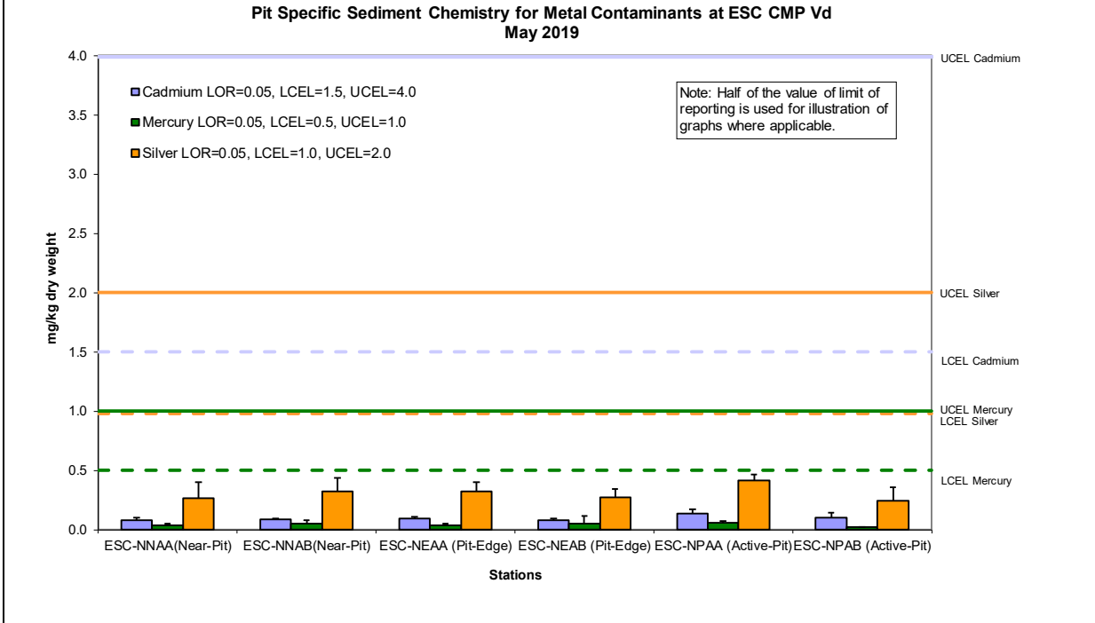
Figure 12: Concentration of Metals (Cd, Hg, Ag; mg/kg dry weight; mean +SD) in sediment samples collected from Pit Specific Sediment Chemistry Monitoring for ESC CMP Vd in May 2019.
