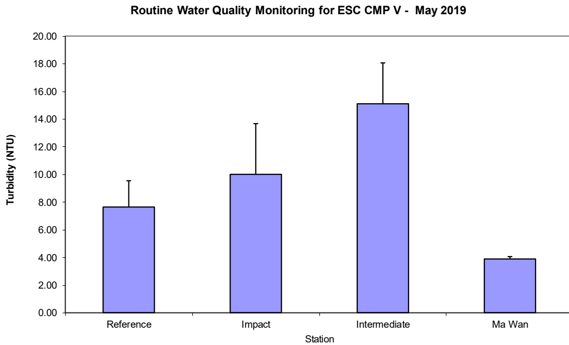
Figure 6: Levels of Turbidity (NTU; mean + SD) recorded during Routine Water Quality Monitoring for disposal operations at ESC CMP V in May 2019.
