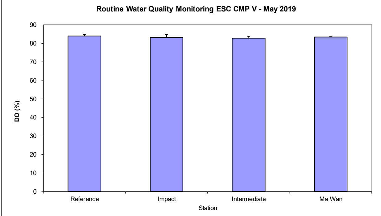
Figure 2: Level of Dissolved Oxygen (DO) (% saturation; mean + SD) recorded during Routine Water Quality Monitoring for disposal operations at ESC CMP V in May 2019.
