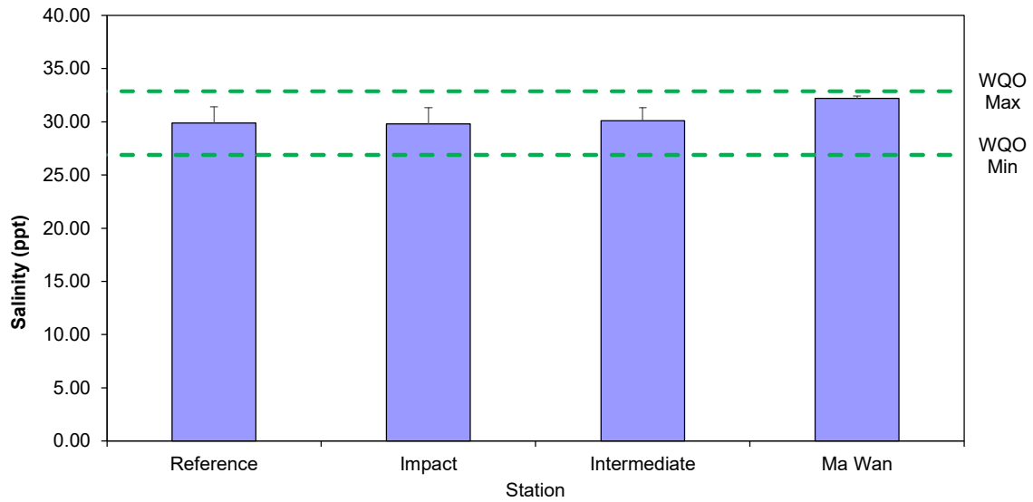
Figure 5: Level of Salinity (ppt; mean + SD 1 ) recorded during Routine Water Quality Monitoring for disposal operations at ESC CMP V in April 2023
