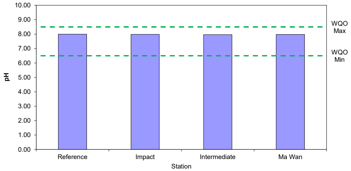
Figure 1: Level of pH recorded during Routine Water Quality Monitoring for disposal operations at ESC CMP V in April 2023
