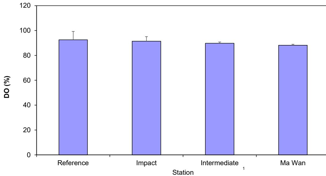
Figure 2: Level of Dissolved Oxygen (DO) (% saturation; mean + SD) recorded during Routine Water Quality Monitoring for disposal operations at ESC CMP V in April 2023
