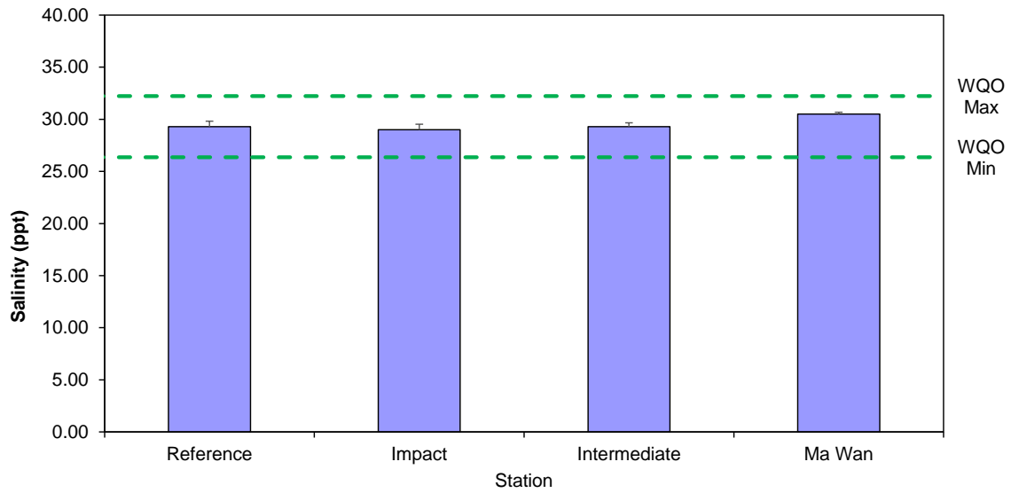
Figure 5: Level of Salinity (ppt; mean + SD 1 ) recorded during Routine Water Quality Monitoring for disposal operations at ESC CMP V in May 2023
