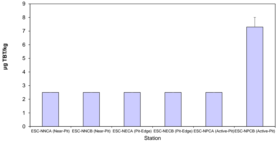
Figure 16: Concentration of Tributyltin (TBT) ( \mu\text{g TBT/kg} ; mean + SD) in sediment samples collected from Pit Specific Sediment Chemistry Monitoring for ESC CMP Vb in May 2023
