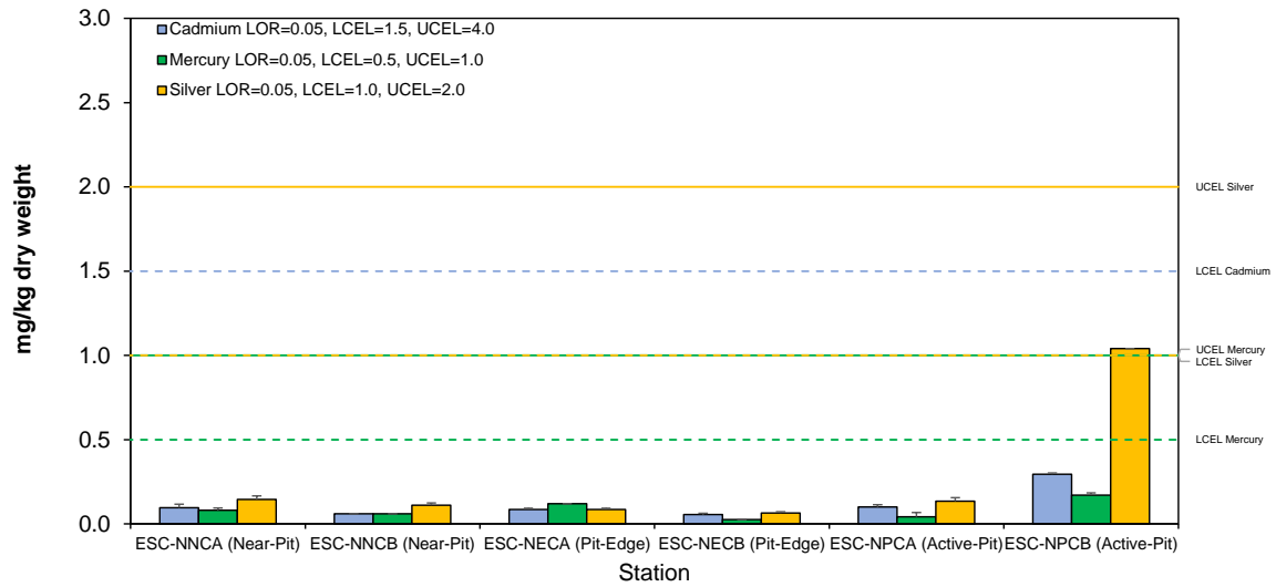
Figure 13: Concentration of Metals (Cd, Hg, Ag; mg/kg dry weight; mean + SD) in sediment samples collected from Pit Specific Sediment Chemistry Monitoring for ESC CMP Vb in May 2023
