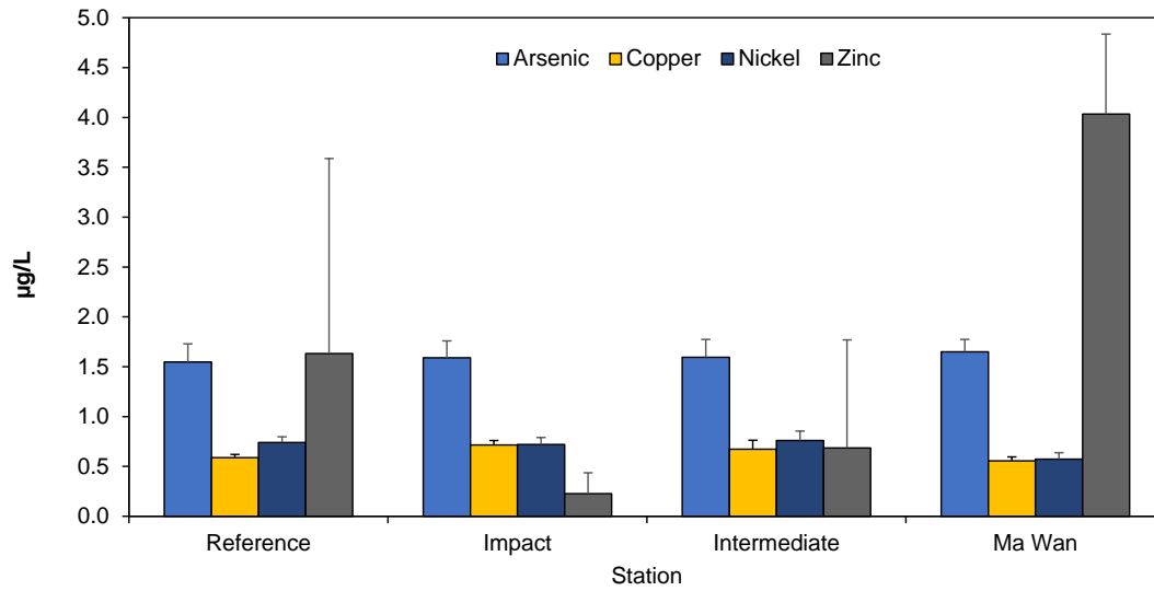
Figure 7: Concentration of Arsenic, Copper, Nickel, and Zinc (µg/L; mean + SD) in water samples collected from Routine Water Quality Monitoring for disposal operations at ESC CMP V in May 2023
