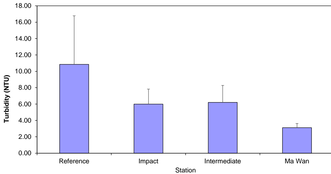
Figure 6: Level of Turbidity (NTU; mean + SD 1 ) recorded during Routine Water Quality Monitoring for disposal operations at ESC CMP V in May 2023
