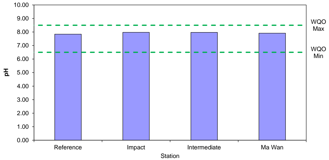
Figure 1: Level of pH recorded during Routine Water Quality Monitoring for disposal operations at ESC CMP V in May 2023
