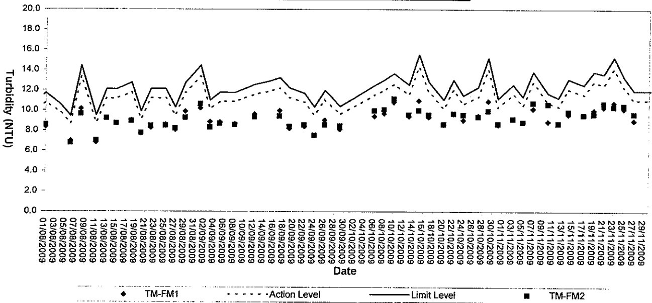
Turbidity (Depth-average) at Mid-Ebb Tide
