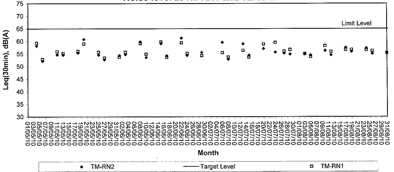
Noise level at TM-RN1 and TM-RN2
