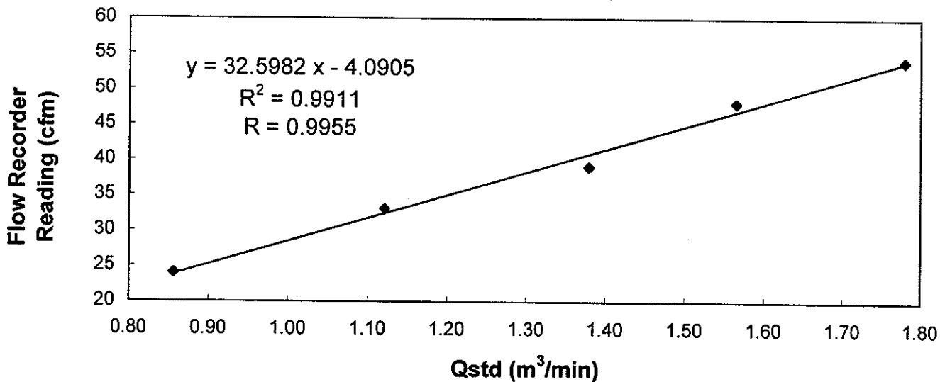
Sampler 9864 Calibration Curve Site: Tuen Mun (A2)
