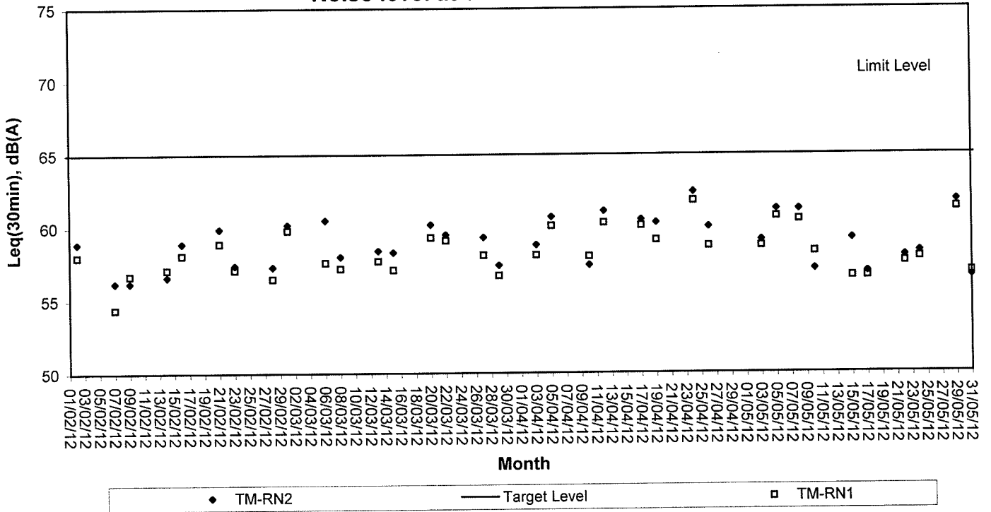
Noise level at TM-RN1 and TM-RN2
