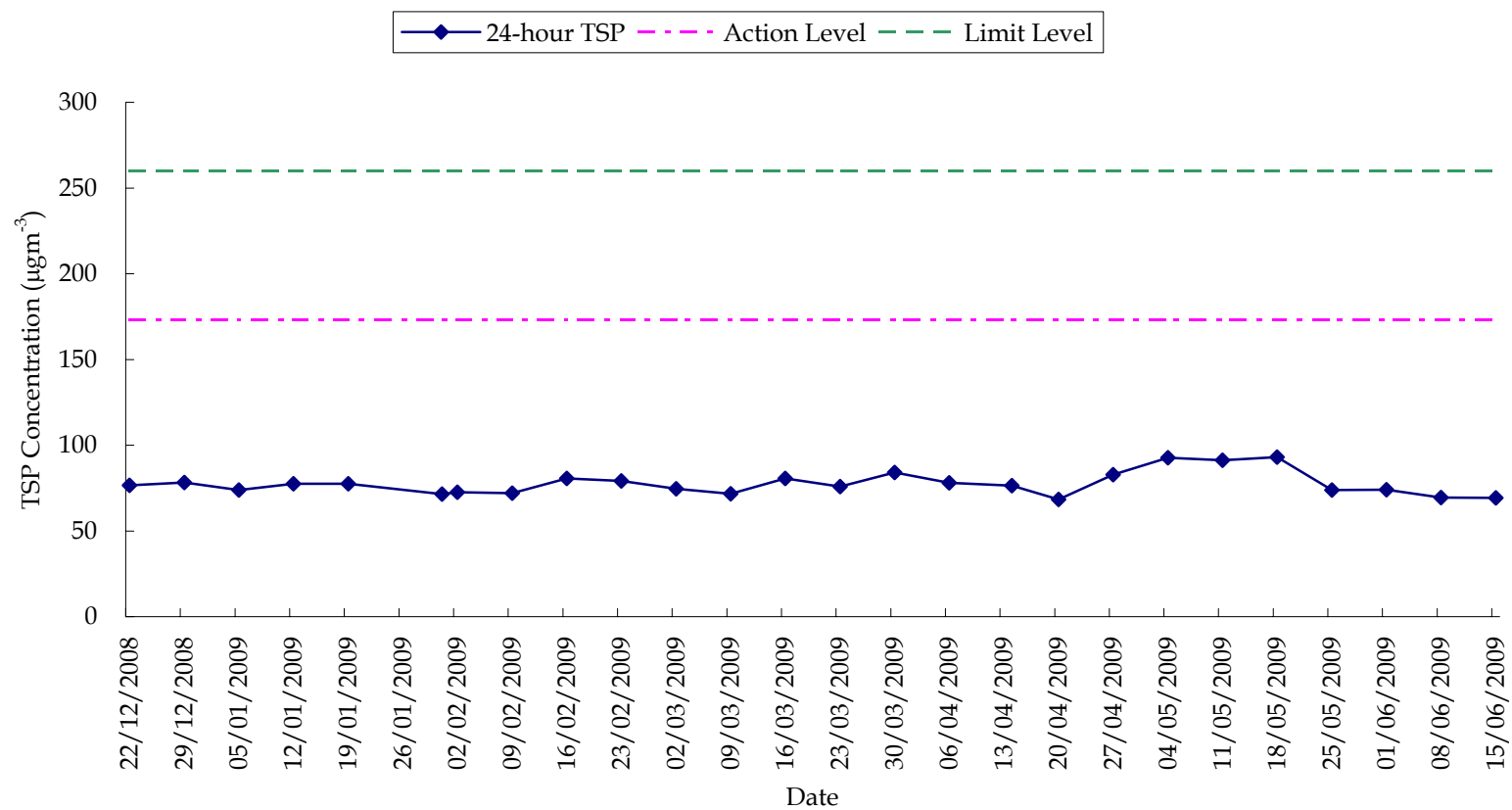
Figure F1 - Measured 24-hour TSP Concentration ( \mu\text{g}\text{m}^{-3} ) at AM1
