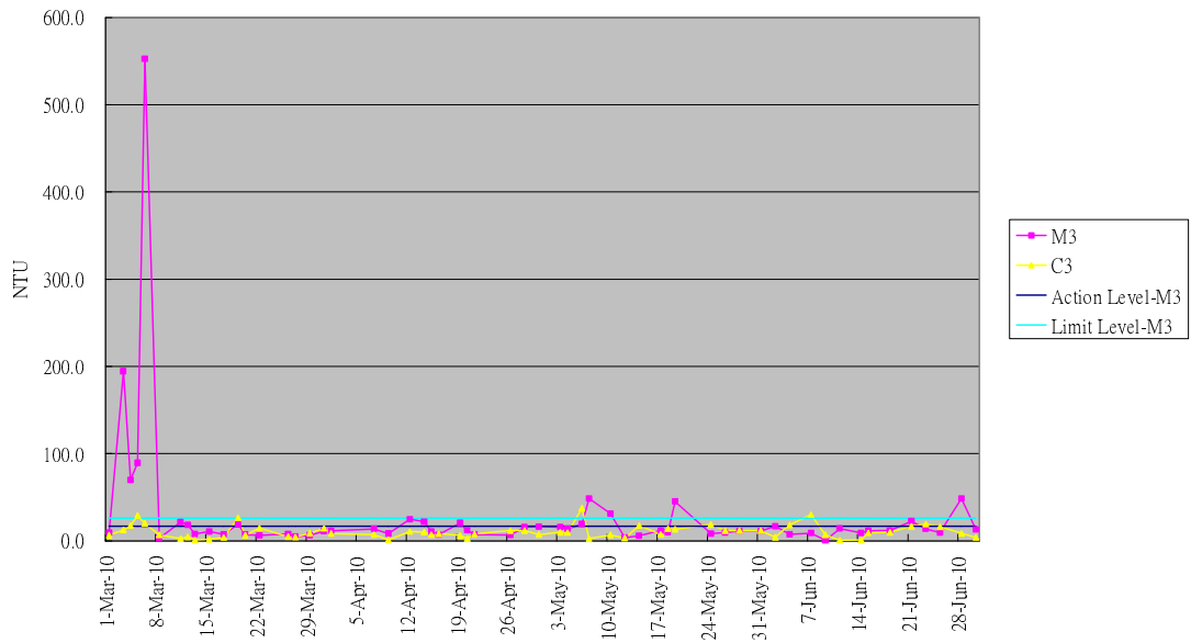
Graphical Plot of Turbidity Trend M3&C3 (Mar - Jun 10)
