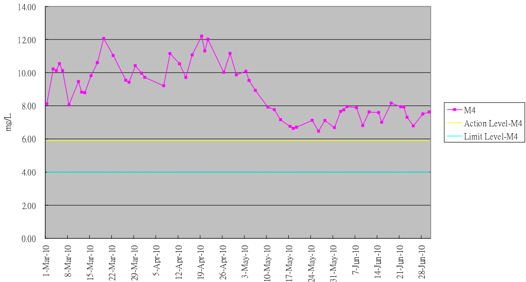
Graphical Plot of Dissolved Oxygen Trend M4 (Mar - Jun 10)
