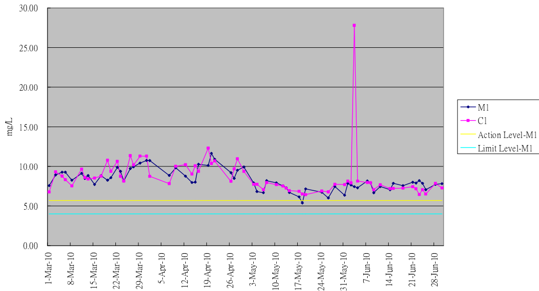
Graphical Plot of Dissolved Oxygen Trend M1&C1 (Mar - Jun 10)
