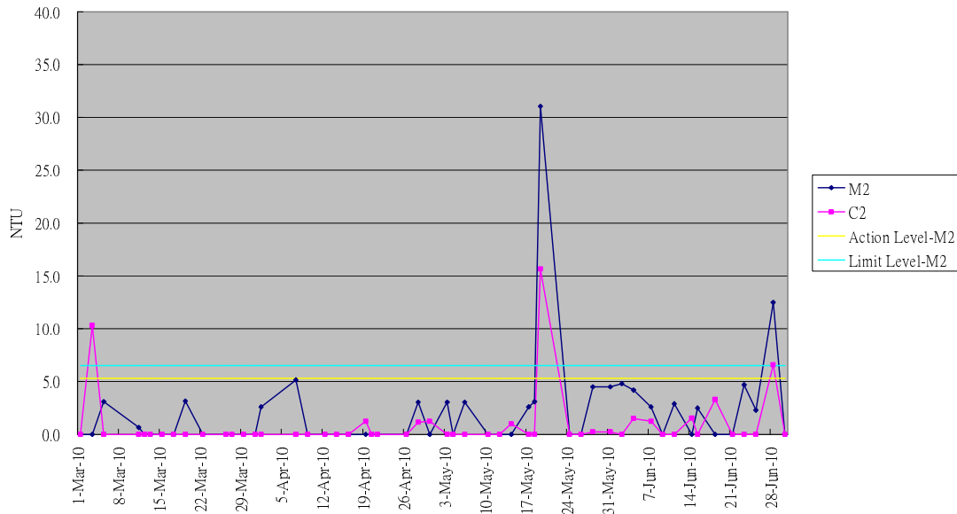
Graphical Plot of Turbidity Trend M2&C2 (Mar - Jun 10)
