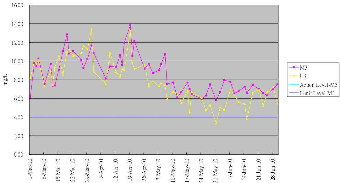
Graphical Plot of Dissolved Oxygen Trend M3&C3 (Mar - Jun 10)
