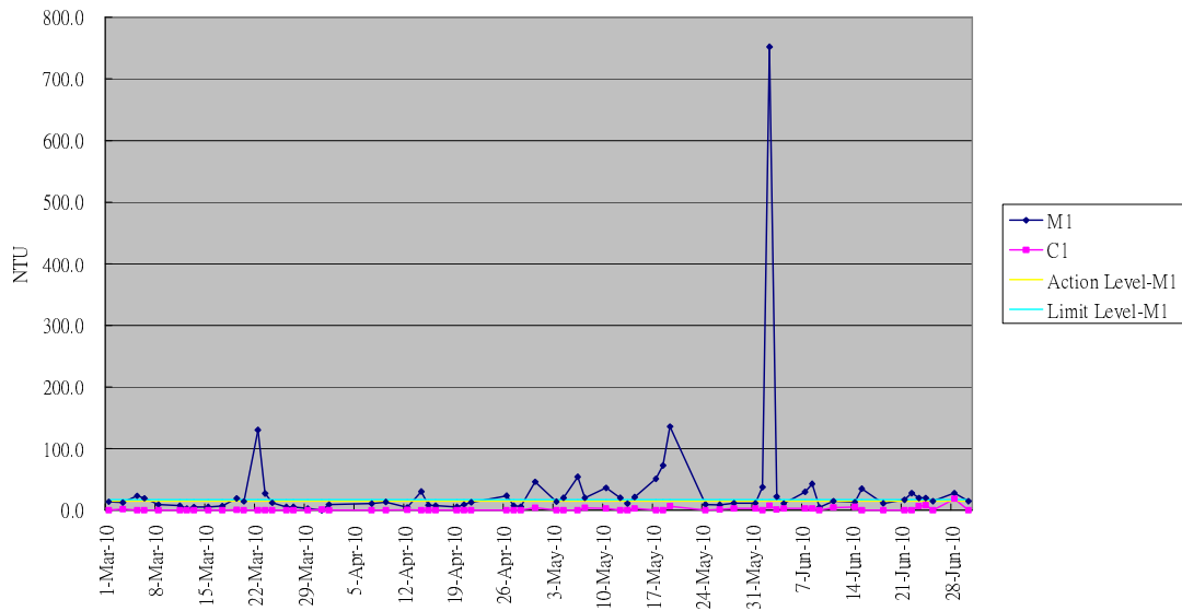
Graphical Plot of Turbidity Trend M1&C1(Mar - Jun 10)
