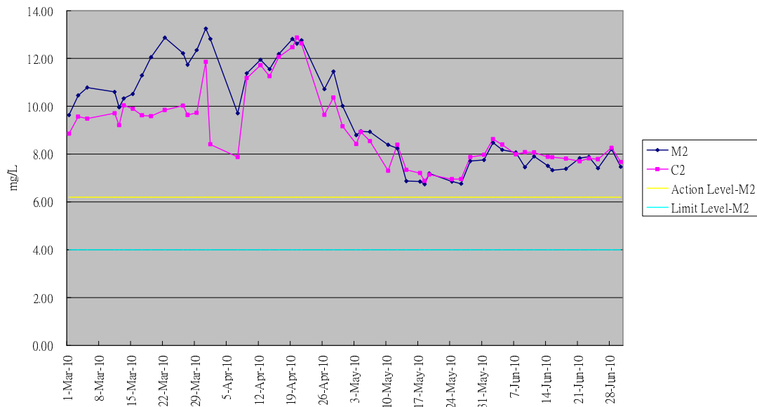
Graphical Plot of Dissolved Oxygen Trend M2&C2 (Mar - Jun 10)
