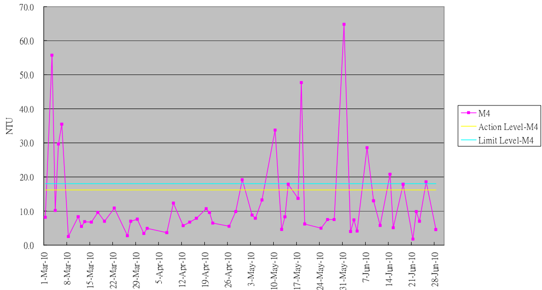
Graphical Plot of Turbidity Trend M4 (Mar - Jun 10)
