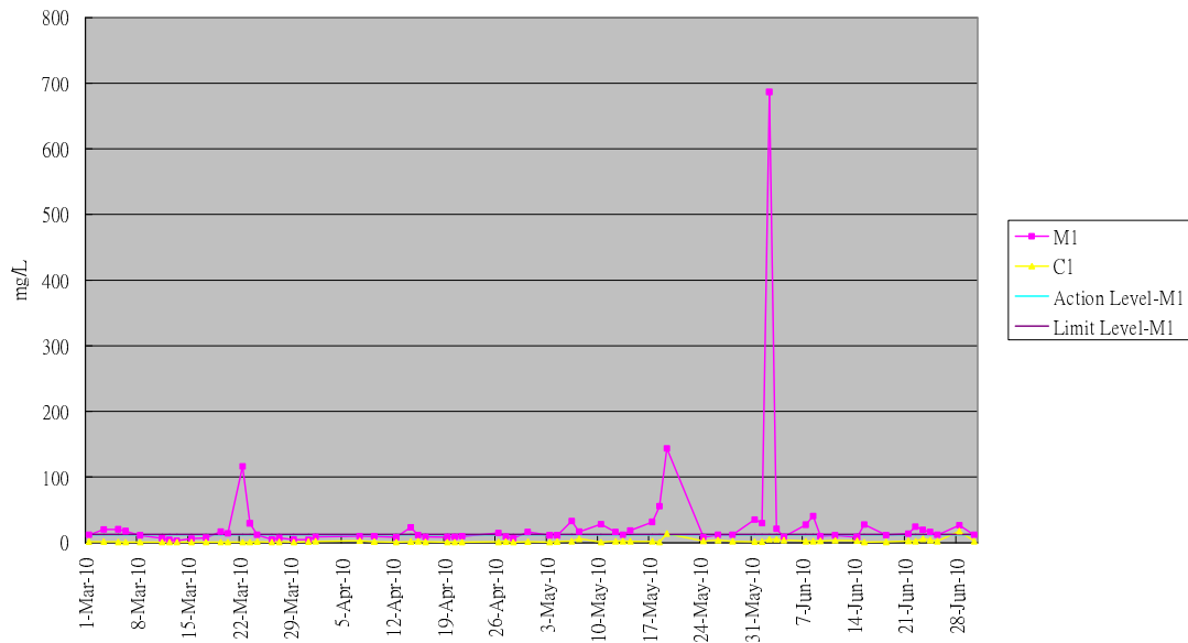
Graphical Plot of Suspended Solid M1&C1 (Mar - Jun 10)
