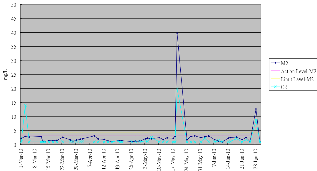
Graphical Plot of Suspended Solid M2&C2 (Mar - Jun 10)
