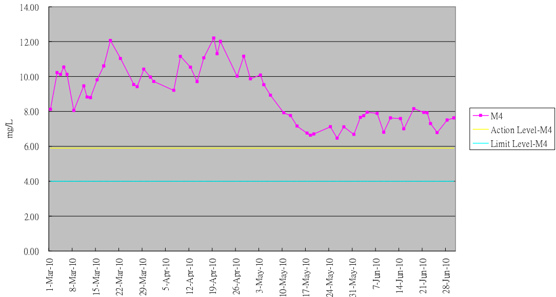
Graphical Plot of Dissolved Oxygen Trend M4 (Mar - Jun 10)
