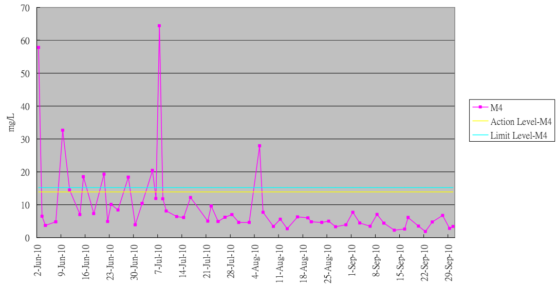
Graphical Plot of Suspended Soild M4 (Jun - Sept 10)
