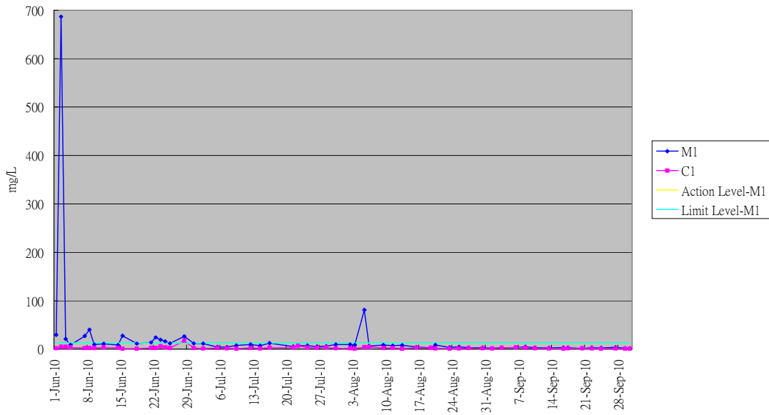
Graphical Plot of Suspended Soild M1&C1 (Jun - Sept 10)
