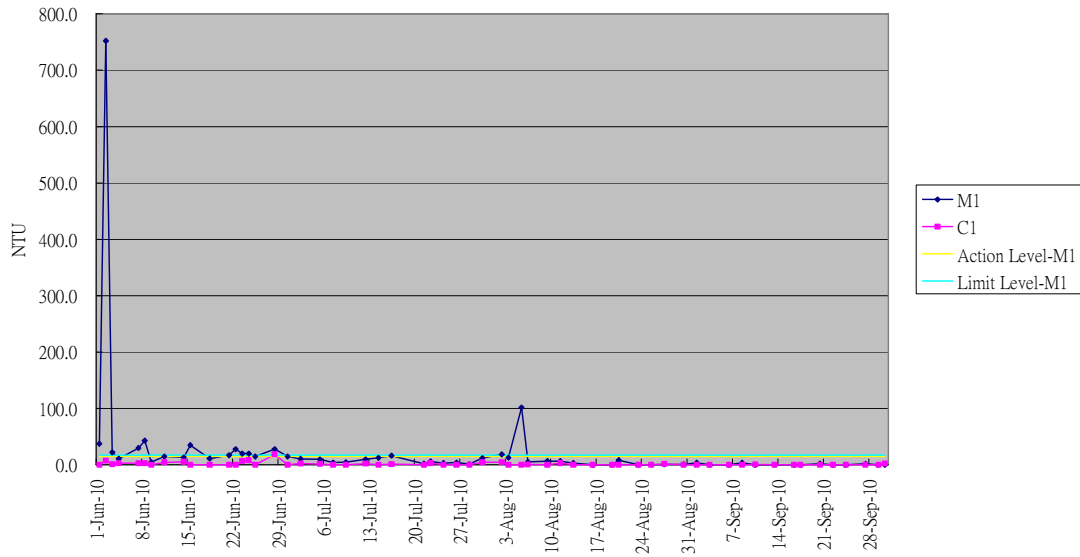
Graphical Plot of Turbidity Trend M1&C1(Jun - Sept 10)
