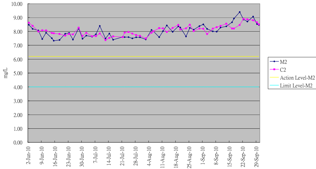
Graphical Plot of Dissolved Oxygen Trend M2&C2 (Jun - Sept 10)
