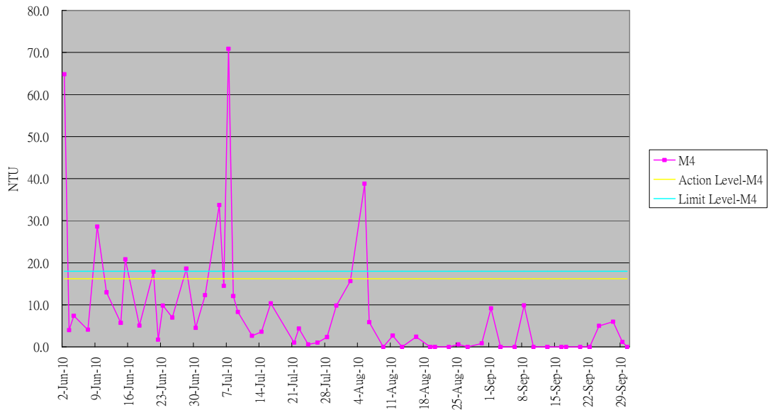
Graphical Plot of Turbidity Trend M4 (Jun - Sept 10)
