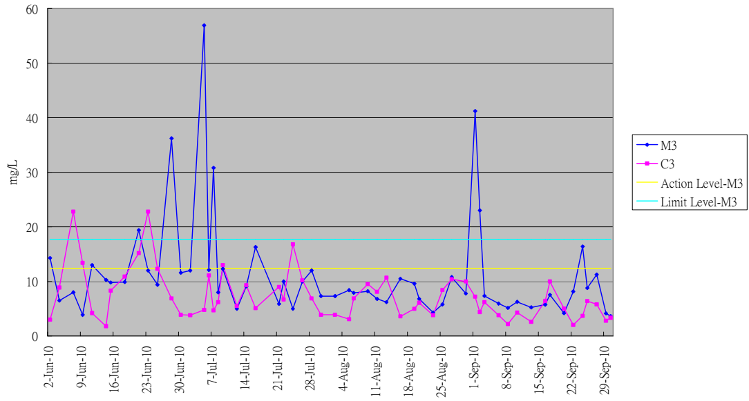
Graphical Plot of Suspended Soild M3&C3 (Jun - Sept 10)
