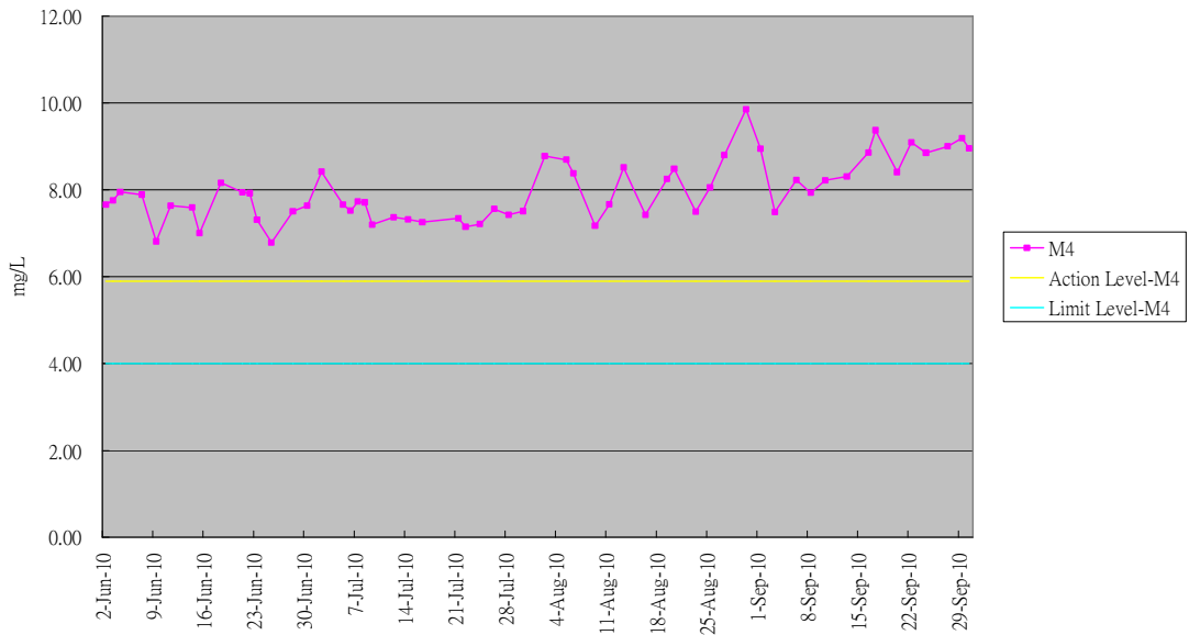
Graphical Plot of Dissolved Oxygen Trend M4 (Jun - Sept 10)
