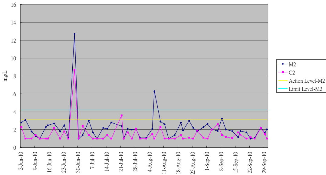
Graphical Plot of Suspended Soild M2&C2 (Jun - Sept 10)
