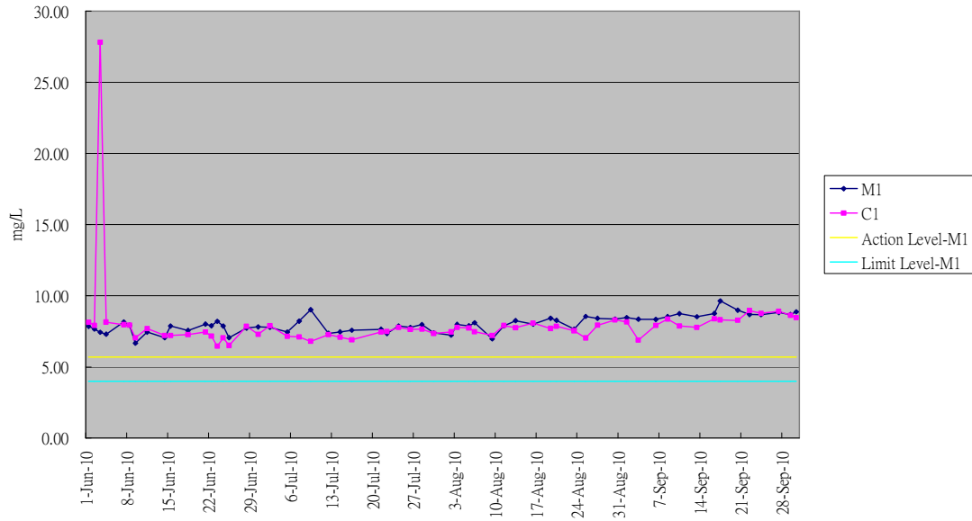
Graphical Plot of Dissolved Oxygen Trend M1&C1 (Jun - Sept 10)
