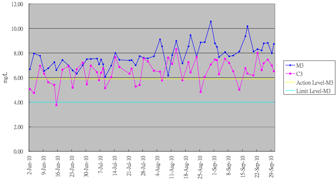
Graphical Plot of Dissolved Oxygen Trend M3&C3 (June - Sept 10)
