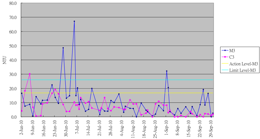
Graphical Plot of Turbidity Trend M3&C3 (Jun - Sept 10)
