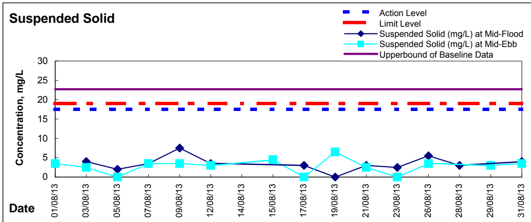
Graphic Presentation of Water Quality Result of WSD15 - Sai Wan Ho with respect to Local Variation
