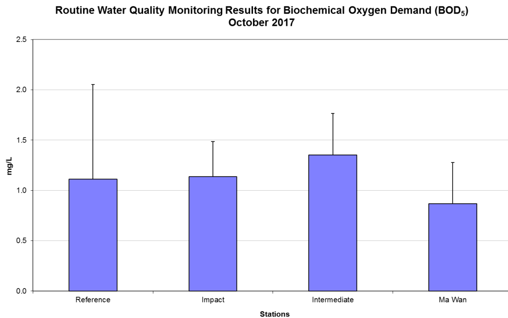
Figure 9: Level of Biochemical Oxygen Demand (BOD 5 ) (mg/L; mean + SD) in water samples collected from Routine Water Quality Monitoring for disposal operations at ESC CMP V in October 2017.
