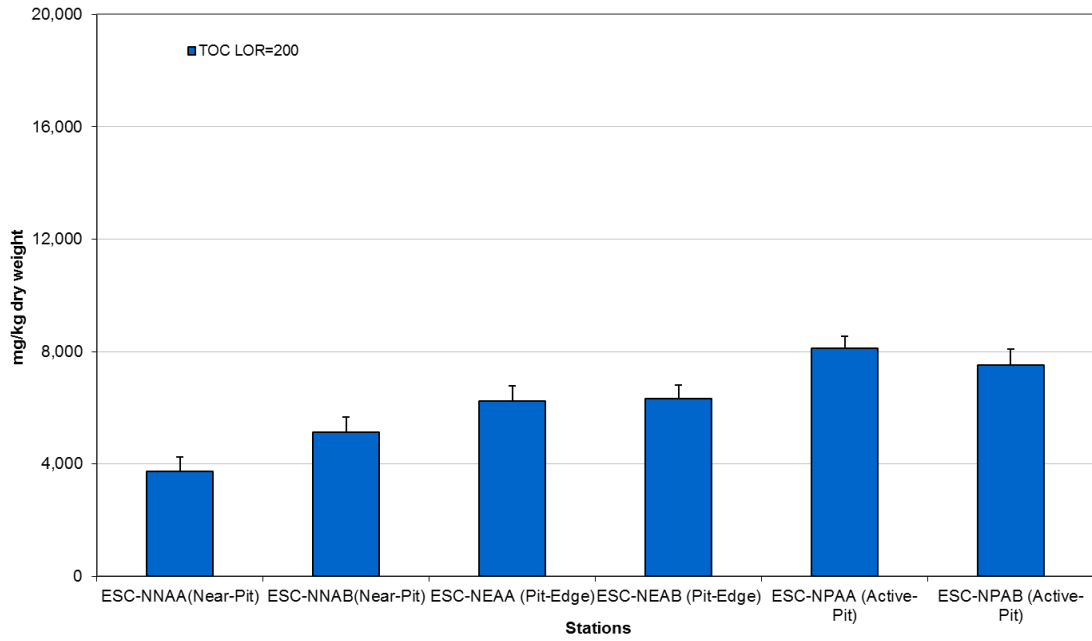
Pit Specific Sediment Chemistry for Total Organic Carbon (TOC) at ESC CMP Vd September 2017
