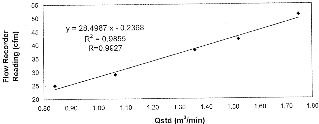
Sampler 9864 Calibration Curve Site: Tuen Mun (A2)
