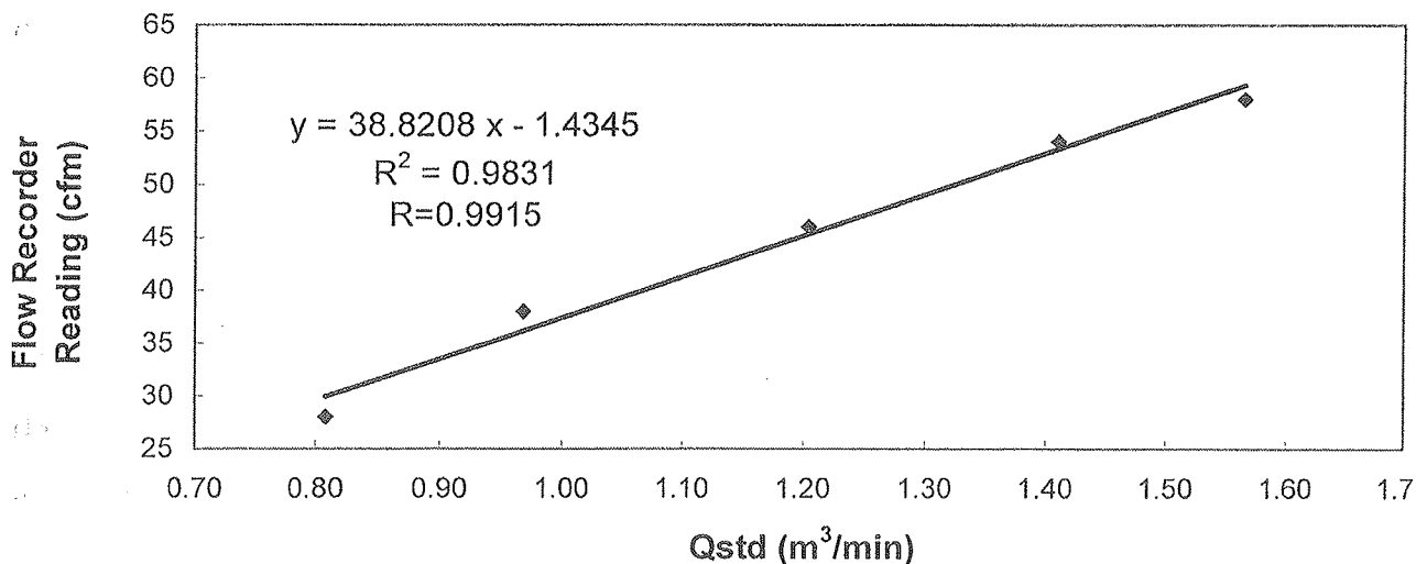
Sampler 10347 Calibration Curve Site: Tuen Mun 38 (TM-A1)
