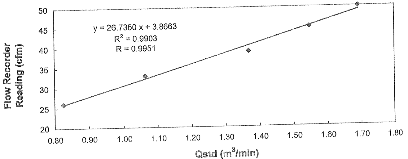
Sampler 9864 Calibration Curve Site: Tuen Mun (TM-RA2)
