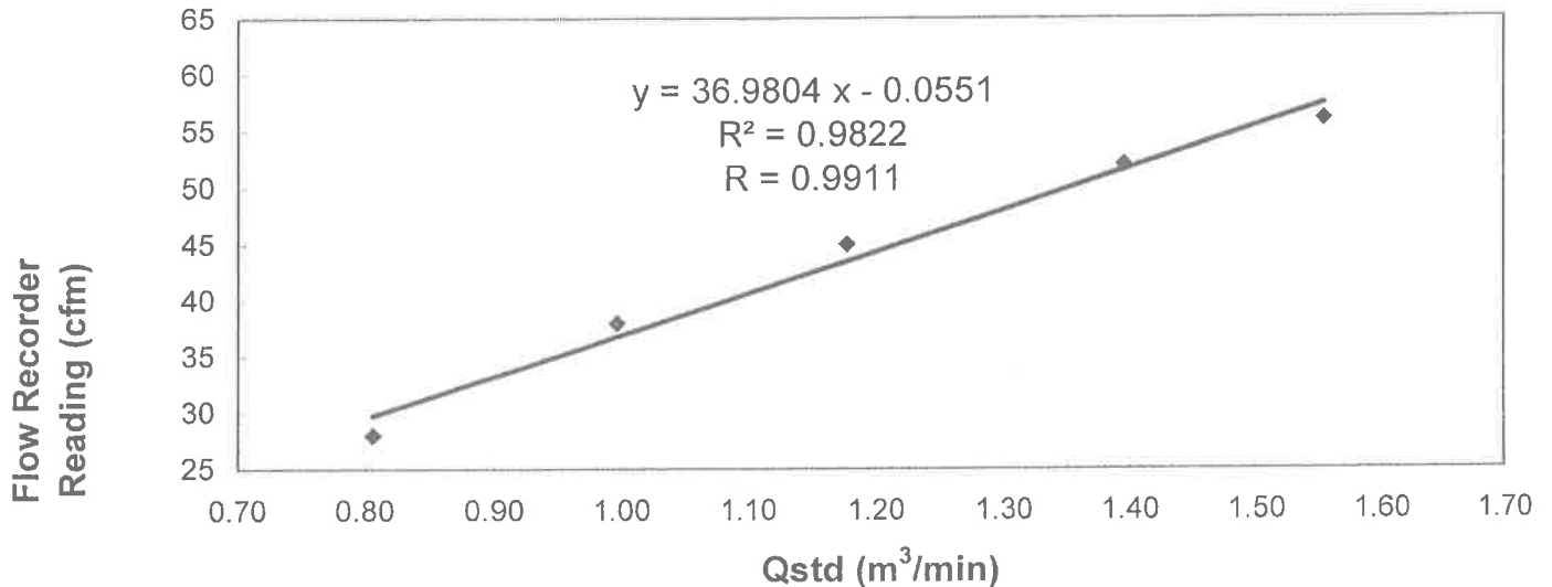
Sampler 10347 Calibration Curve Site: Tuen Mun 38 (TM-A1)
