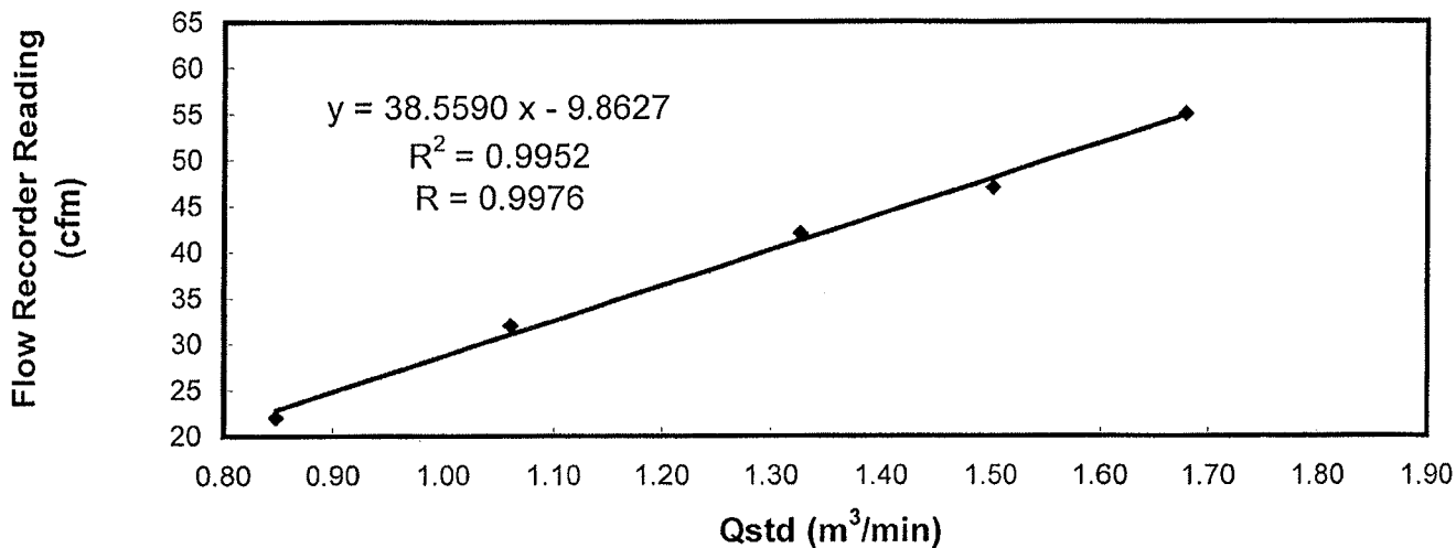
Sampler 1180 Calibration Curve Site: Tuen Mun 38 (TM-RA2)
