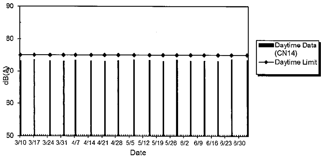
WIL-CN14 Noise Level at Bon-Point, Mar 2014 - Jul 2014
