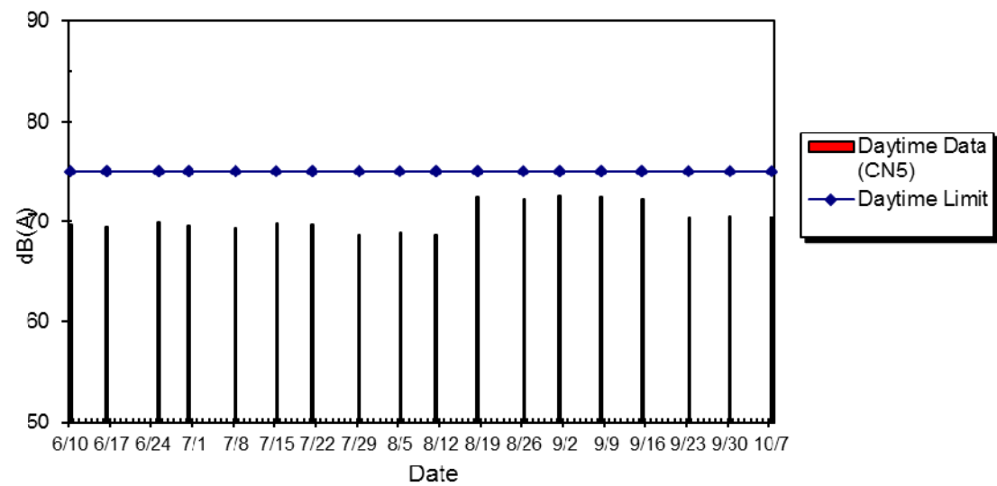
WIL-CN5 Noise Level at Western Court, Jun 2014 - Oct 2014
