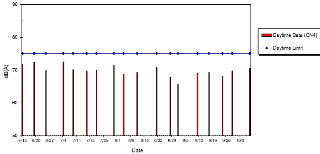
WIL-CN4 Noise Level at Luen Tak Apartments, Jun 2014 - Oct 2014
