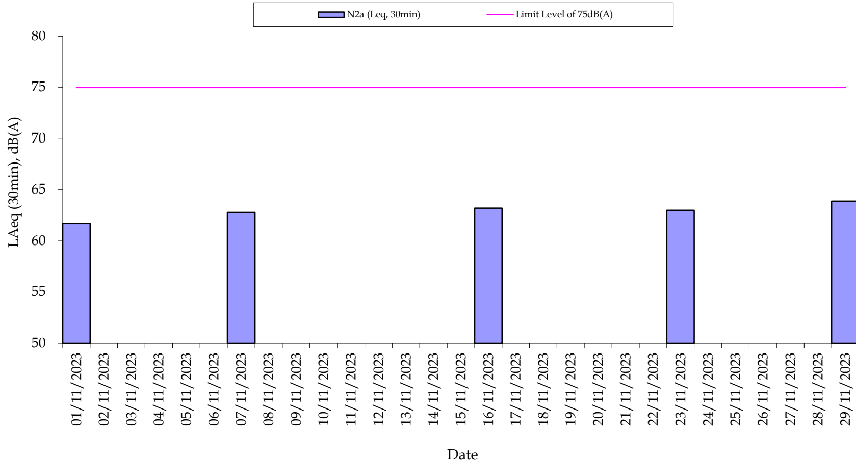
Normal Weekdays Noise Monitoring Results at 2nd Floor of Block 3 at Tai Kwun (N2a) (Leq, 30min)
