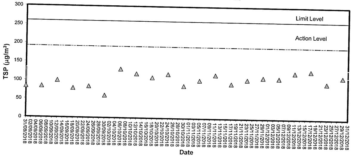
24-hour TSP level at TM-A1
