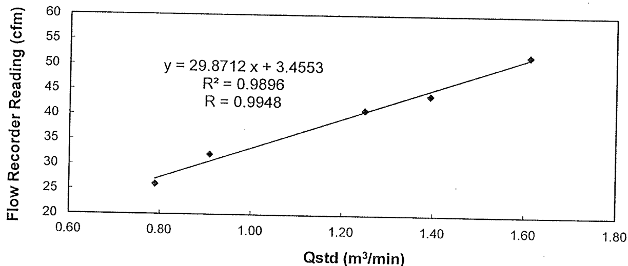
Sampler 2484 Calibration Curve Site: Tuen Mun 38 (TM-A1)
