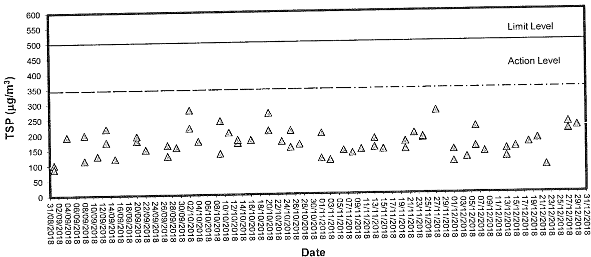
1-hour TSP level at TM-RA2
