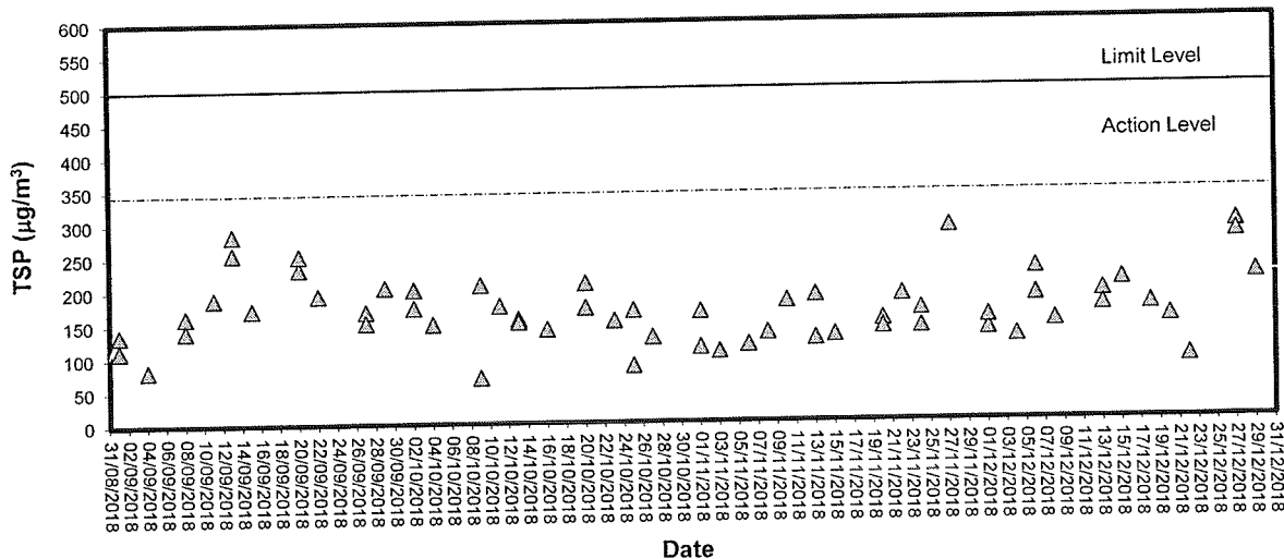
1-hour TSP level at TM-A1
