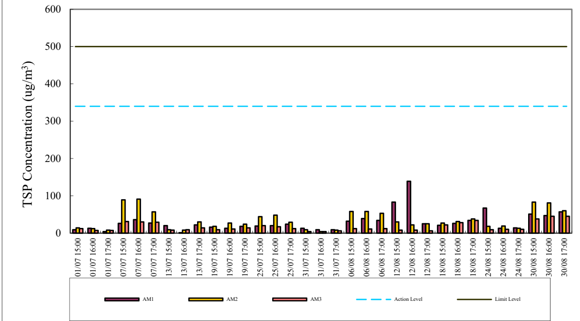
1-hr TSP Air Monitoring Data (July 2023 - August 2023)
