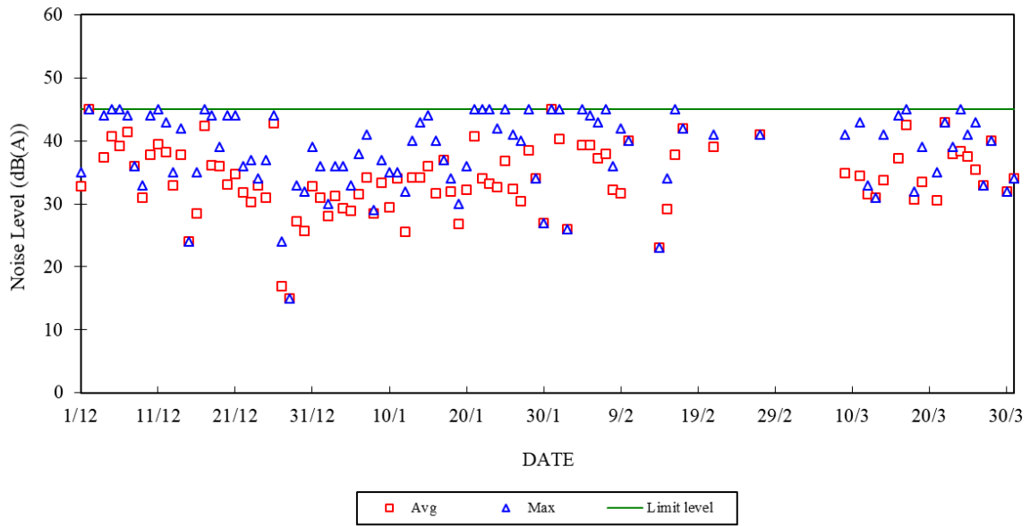
Construction Noise Monitoring in December 2023 - March 2024 NSR at Long Tsai Tsuen/Hung Shing Ye 23:00-07:00 hrs of Next Day
