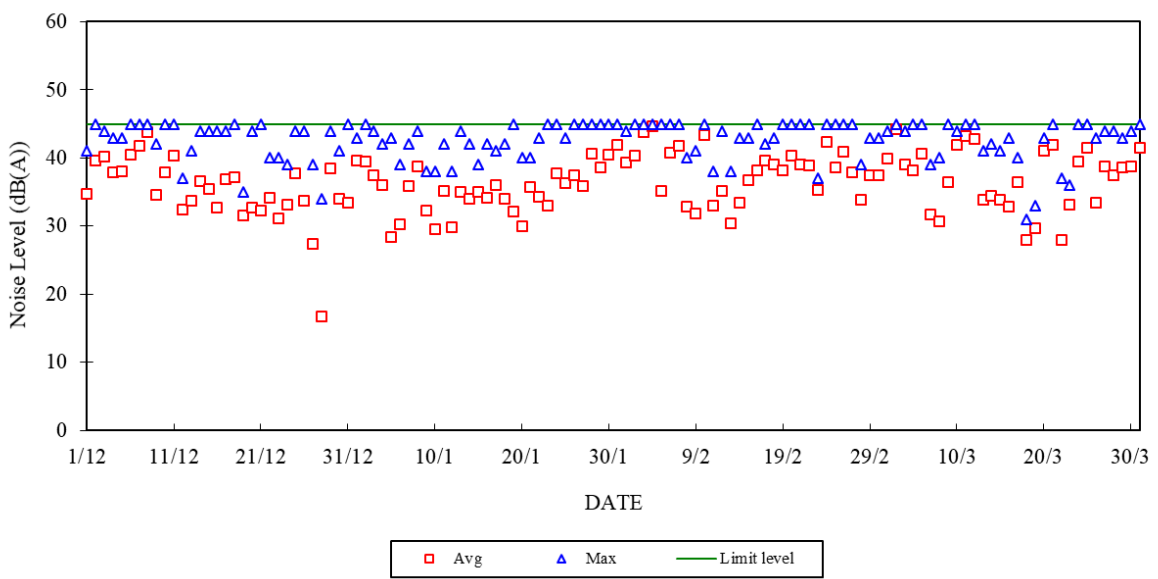
Construction Noise Monitoring in December 2023 - March 2024 NSR at School within Tai Wan San Tsuen 23:00-07:00 hrs of Next Day
