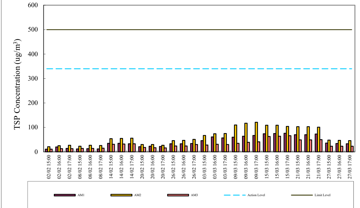
1-hr TSP Air Monitoring Data (February 2024 - March 2024)
