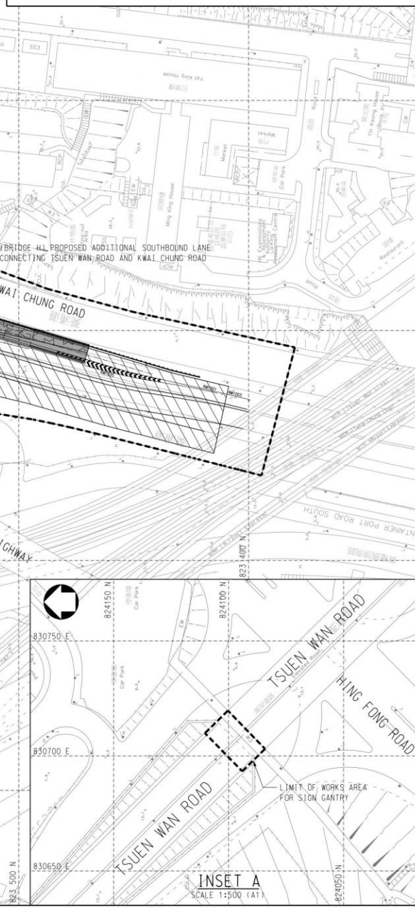
Figure 1.1 Project Layout
