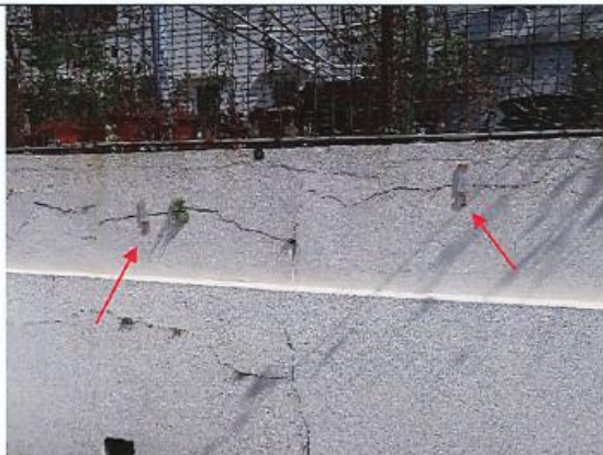
Photo 5: Tell-tales for crack monitoring were installed on the fence wall at NP-10.
