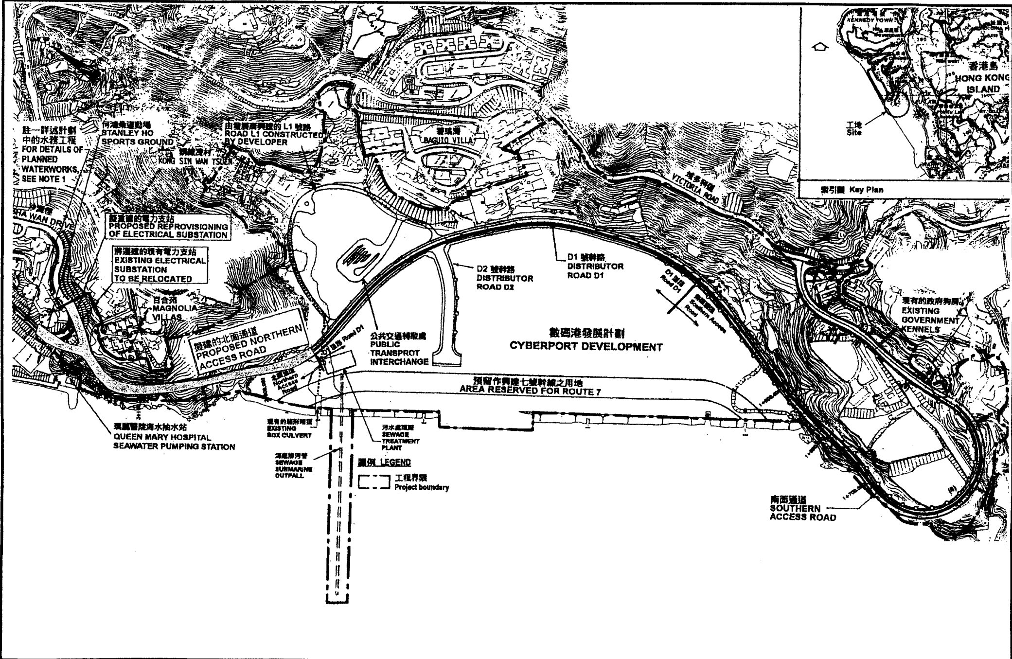
FIGURE 1: ENGINEERING INFRASTRUCTURE FOR CYBERPORT DEVELOPMENT AT TELEGRAPH BAY
