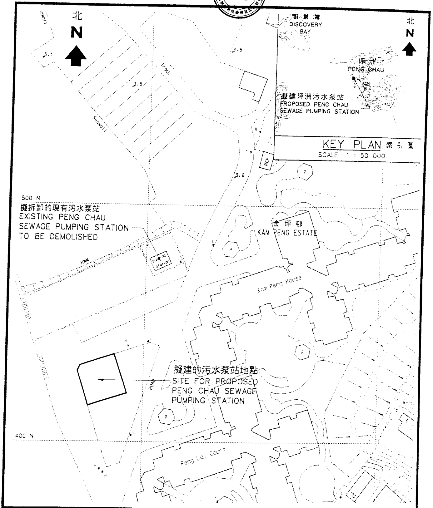
Figure 1 – Location of Peng Chau Sewage Pumping Station Replacement
