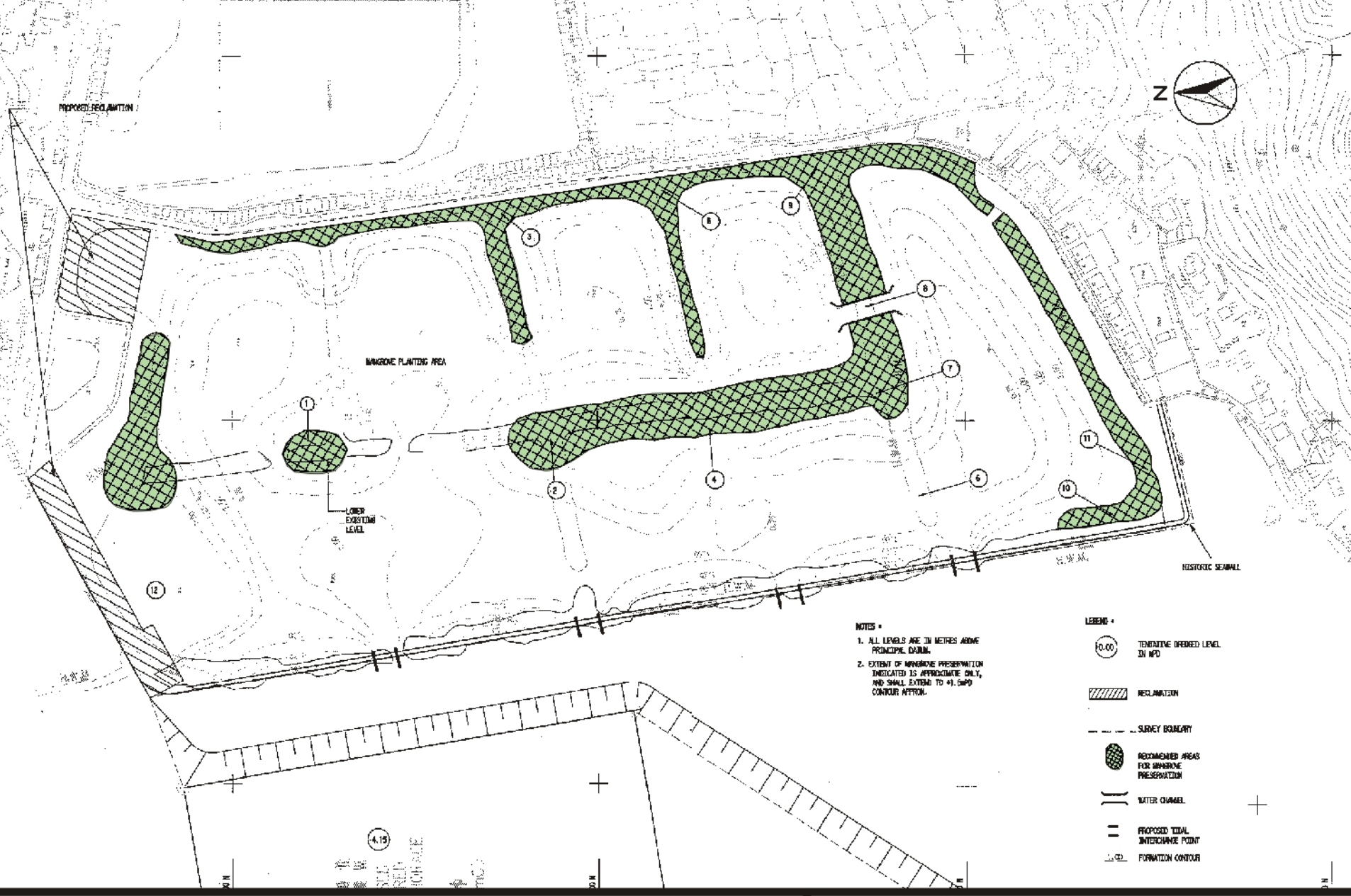
Figure 3 Mangrove Formation Plan
