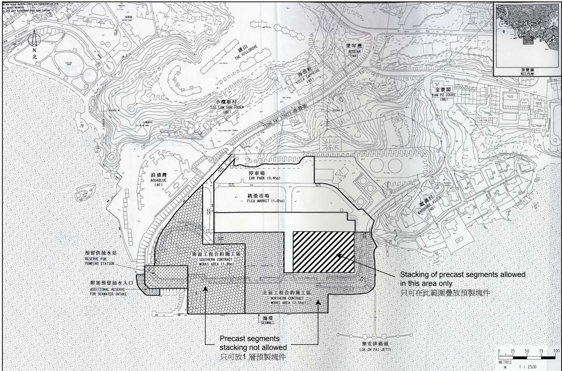
Deep Bay Link and Widening of Yuen Long Highway between Lam Tei and Shap Pat Heung Interchange (Lam Tei to Tan Kwai Tsuen Section) - Works Areas and Barging Point at Lok On Pai (Alternative Plan)
