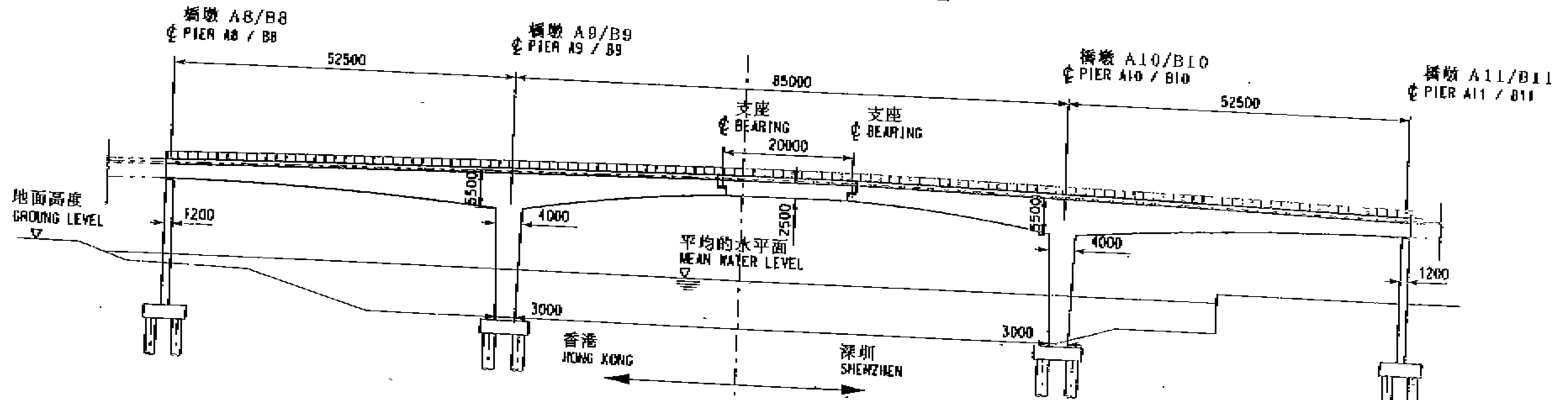
由東面觀望的立面圖 ELEVATION VIEWING FROM EAST
