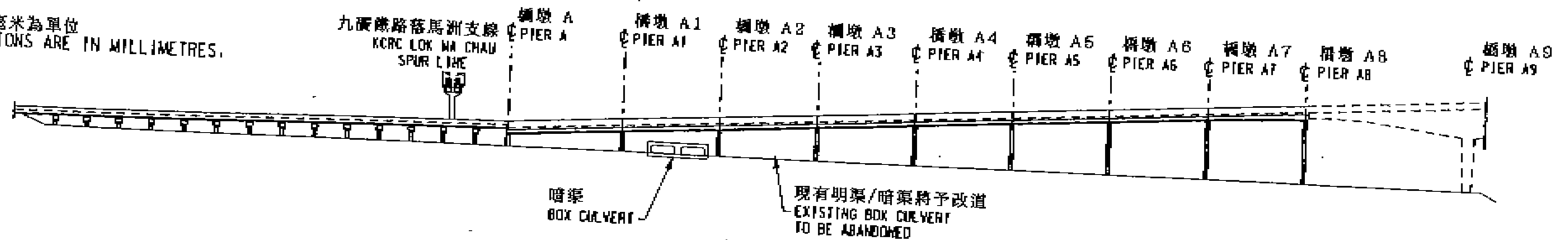
由東面觀望的立面圖 ELEVATION VIEWING FROM EAST
