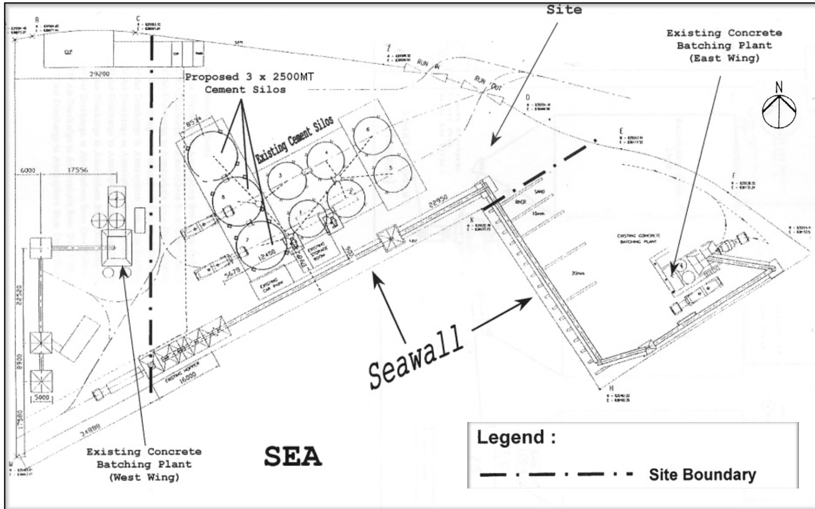
Figure 2 Site Layout Plan for Cement Depot (Extracted from Figure 2.4 of the EIA Report)
