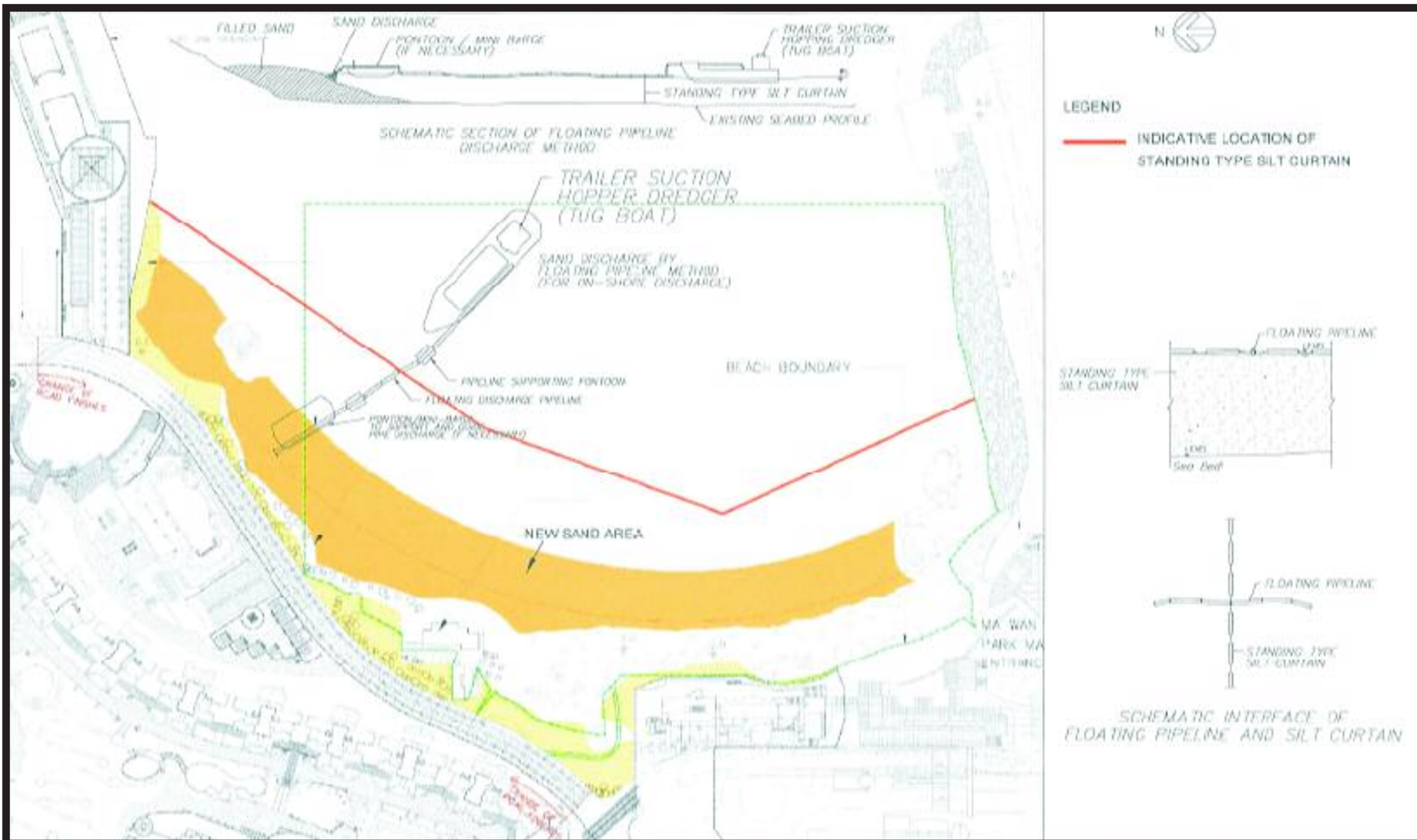
Figure 2 Sand Filling Schematic Layout (Floating Pipeline Method)
