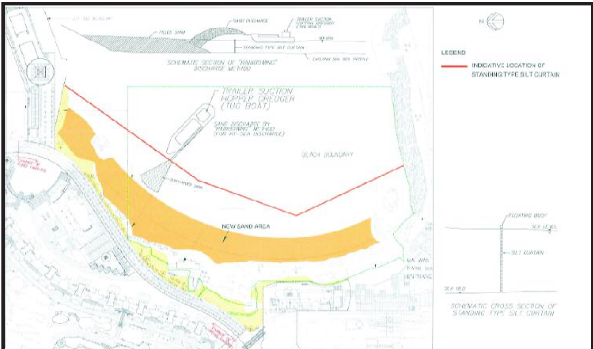
Figure 3 Sand Filling Schematic Layout ("Rainbowing" Method)
