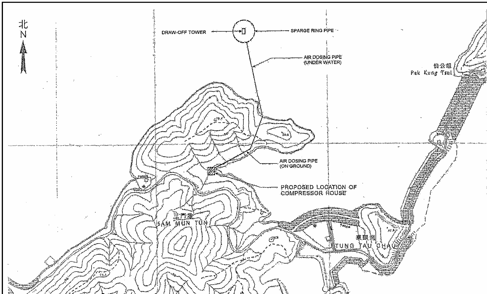
Figure 1 : De-stratification of Plover Cove Reservoir by Aeration — Location Plan
