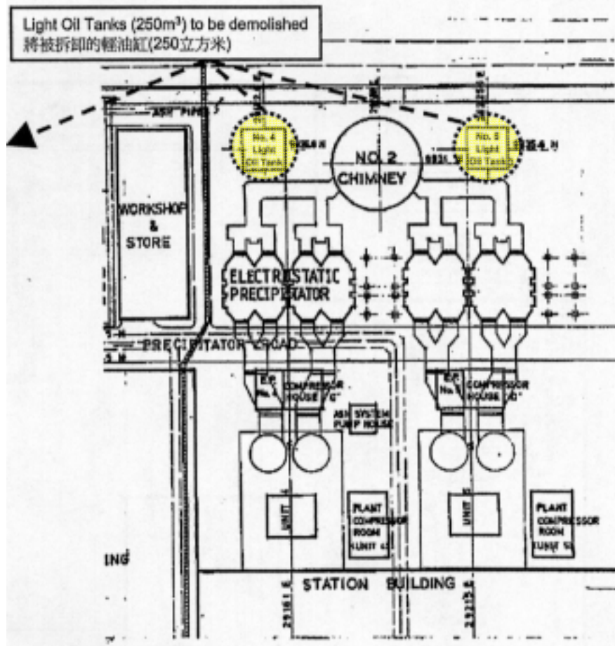
Figure 2: Location of No. 4 and No. 5 Light Oil Tanks 圖 2：四號及五號輕油缸的位置圖
