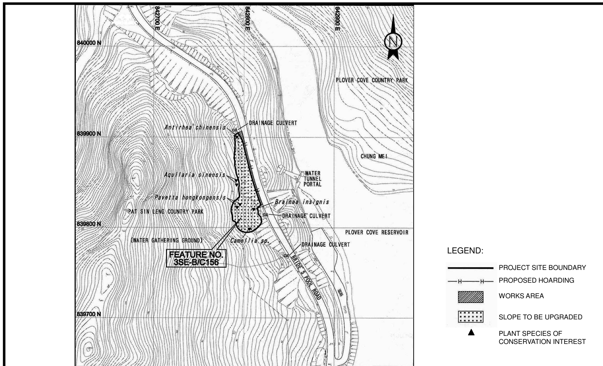
Figure 1 Landslip Preventive Works at Feature No. 3SE-B/C156 Along Bride's Pool Road, Near Chung Mei Plover Cove Reservoir, Tai Po (人造斜坡編號 3SE-B/C 156 的防止山泥傾瀉工程在大埔涌尾近船灣淡水湖，新娘潭路旁)
